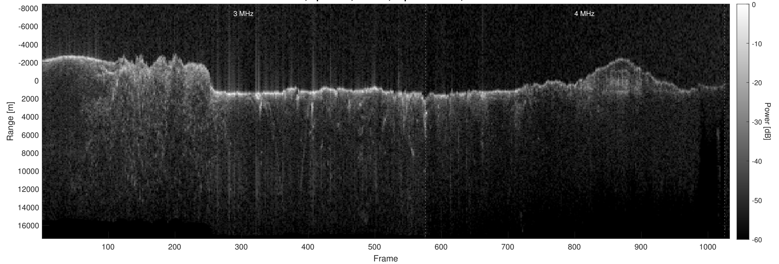
Orbit 6791, Optimized, Window, Depth-Corrected, Channel 2
