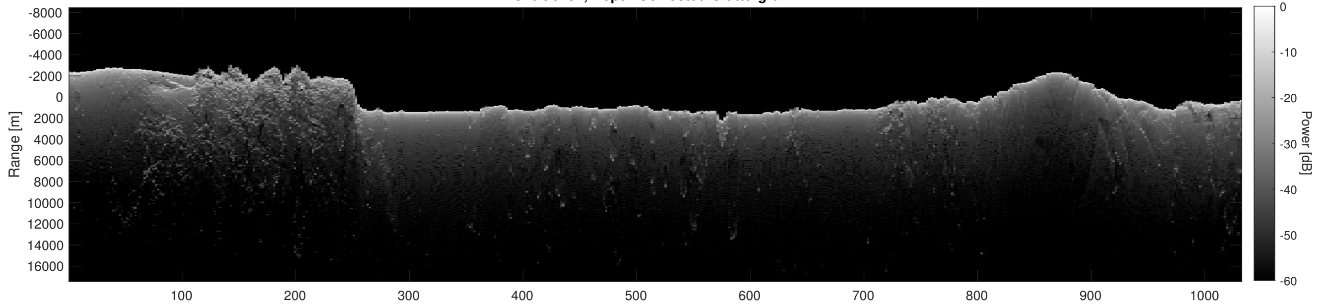
Orbit 6791, Depth-Corrected Cluttergram
