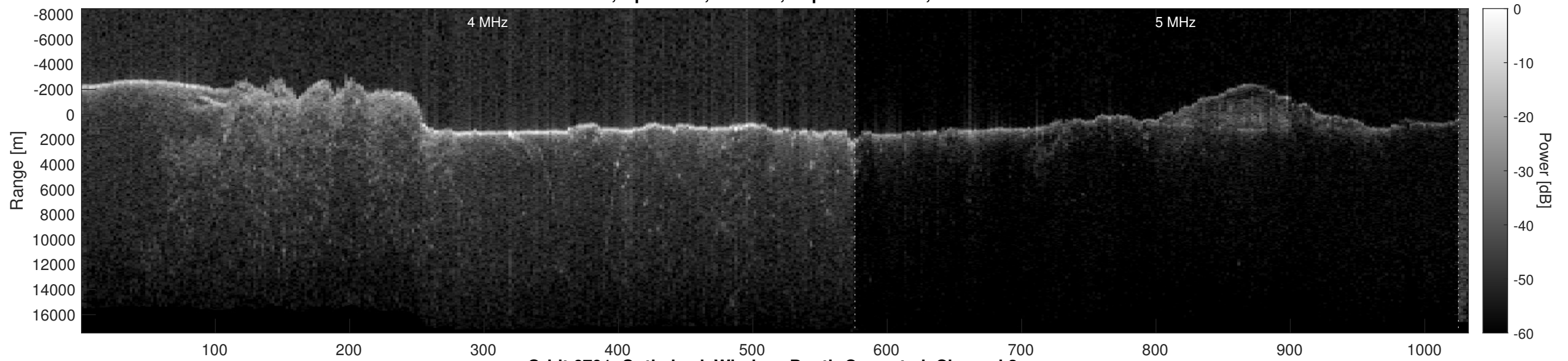
Orbit 6791, Optimized, Window, Depth-Corrected, Channel 2
