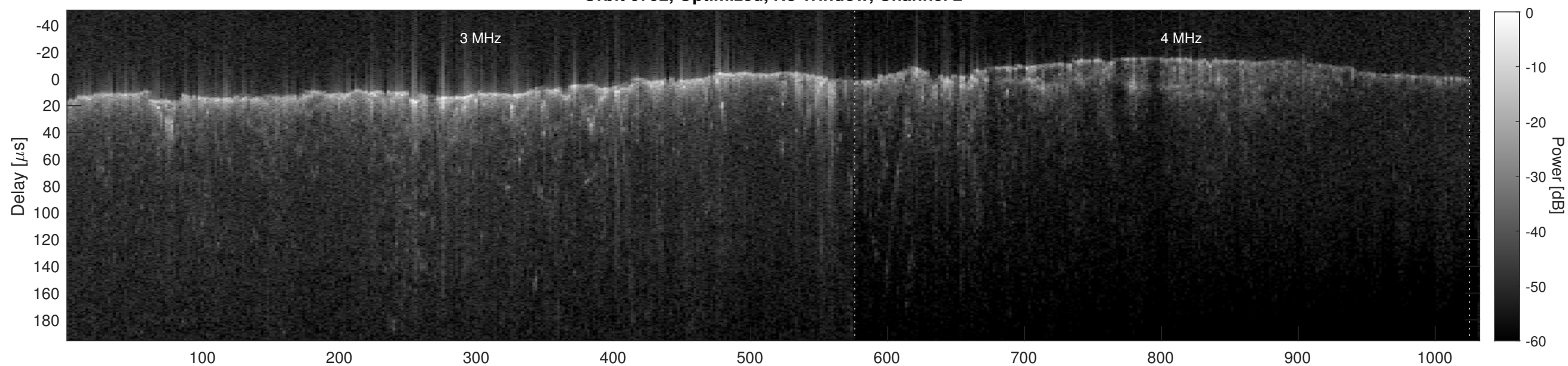
Orbit 6792, Cluttergram
