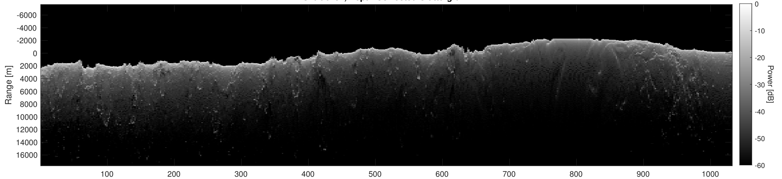
Orbit 6792, Depth-Corrected Cluttergram
