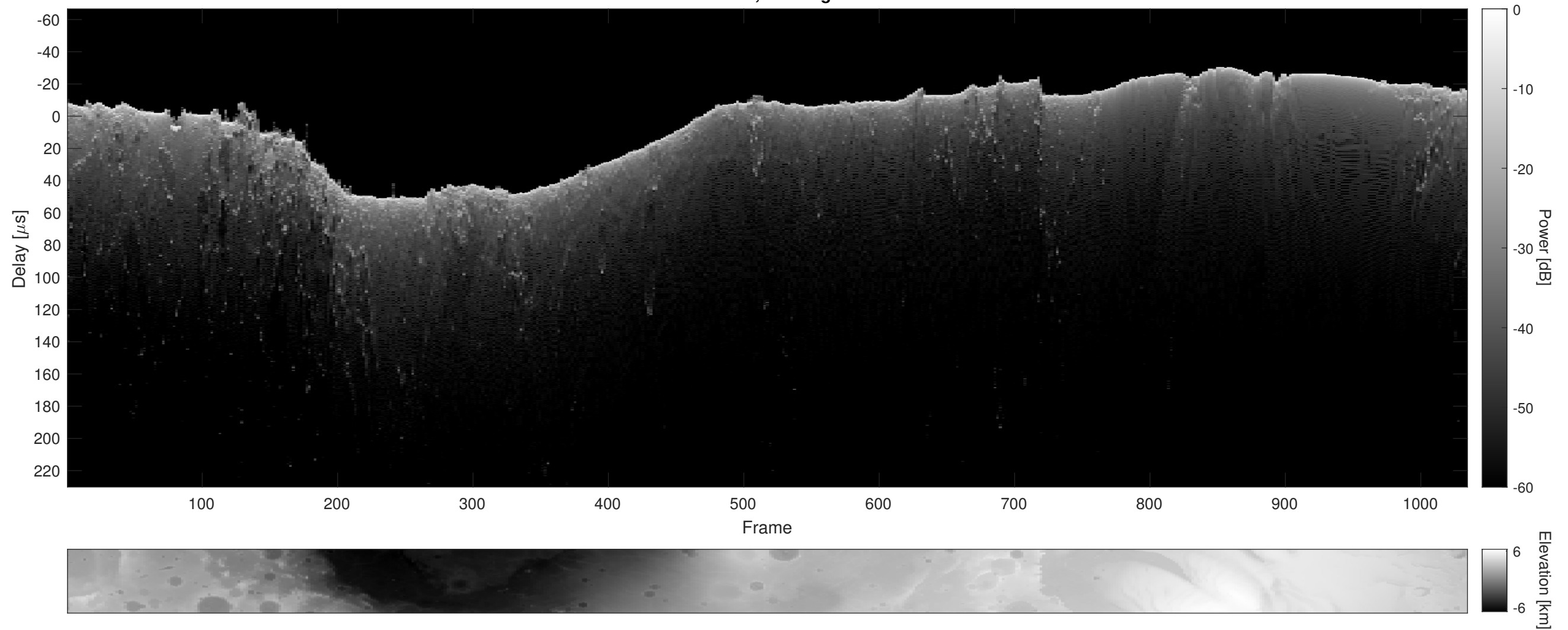
Orbit 6793, Cluttergram
