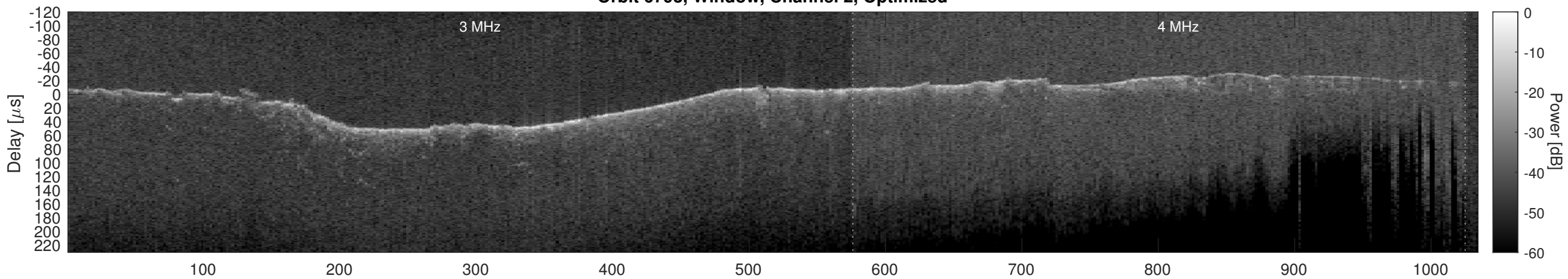
Orbit 6793, Cluttergram
