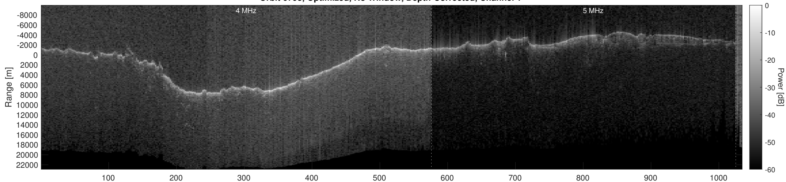
Orbit 6793, Optimized, No Window, Depth-Corrected, Channel 2
