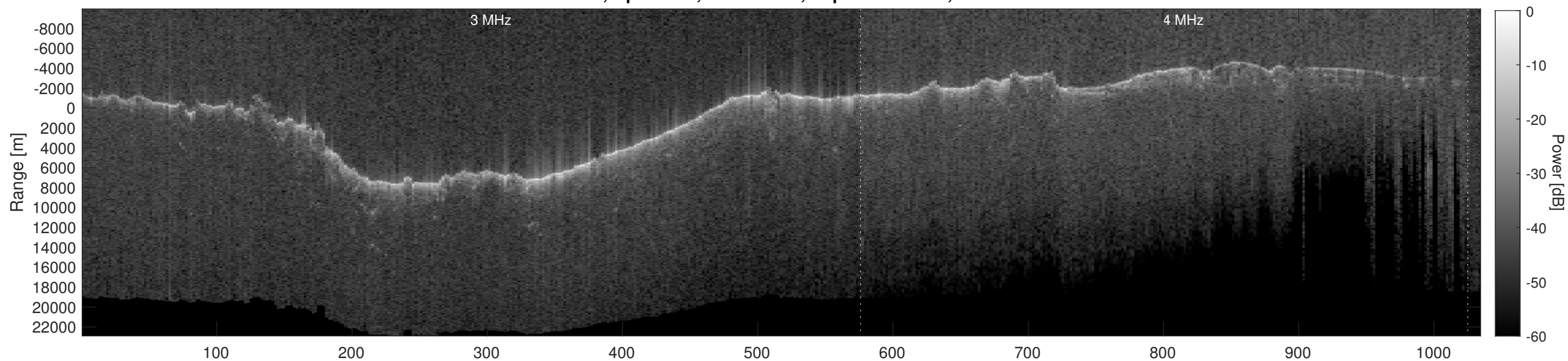
Orbit 6793, Depth-Corrected Cluttergram
