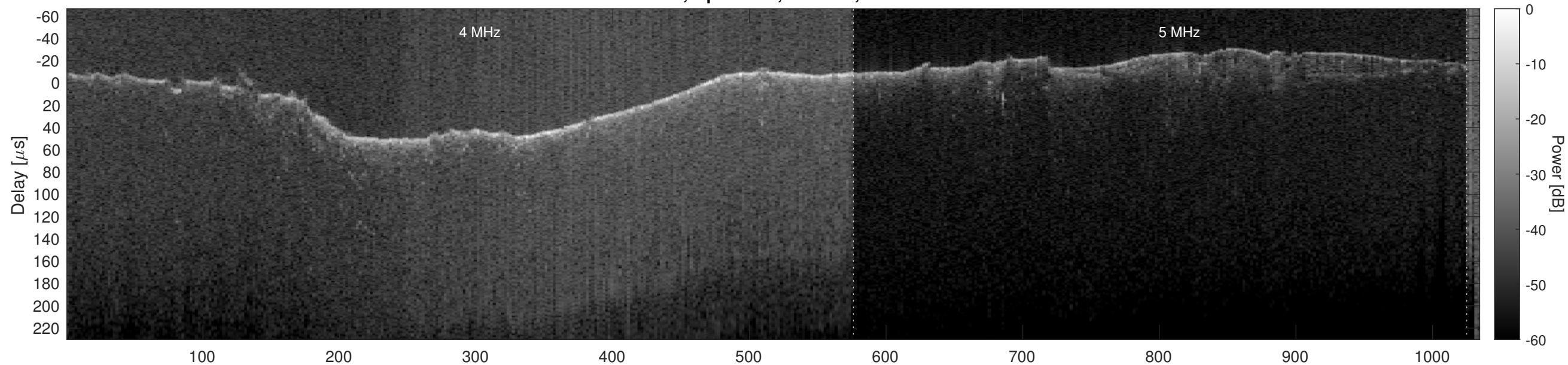
Orbit 6793, Optimized, Window, Channel 2
