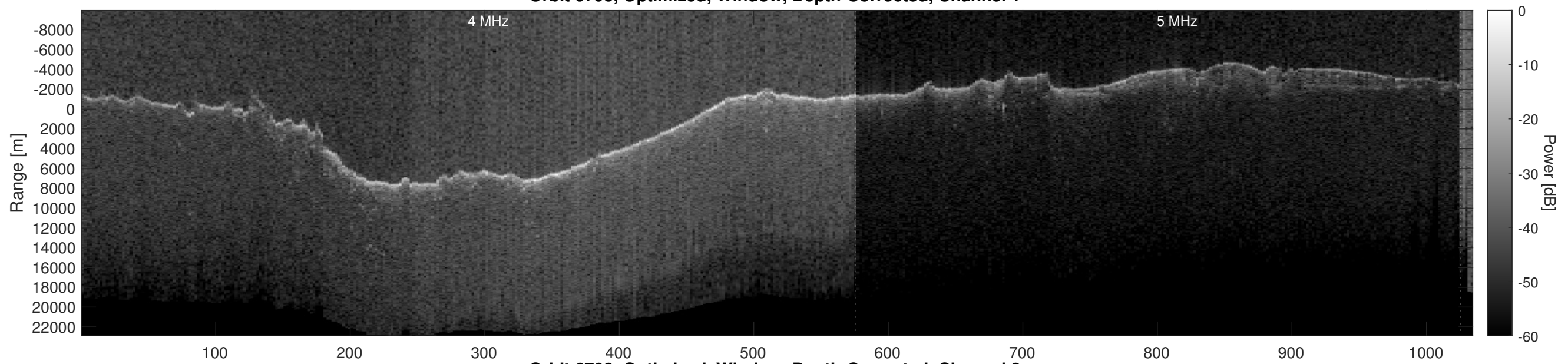
Orbit 6793, Optimized, Window, Depth-Corrected, Channel 2
