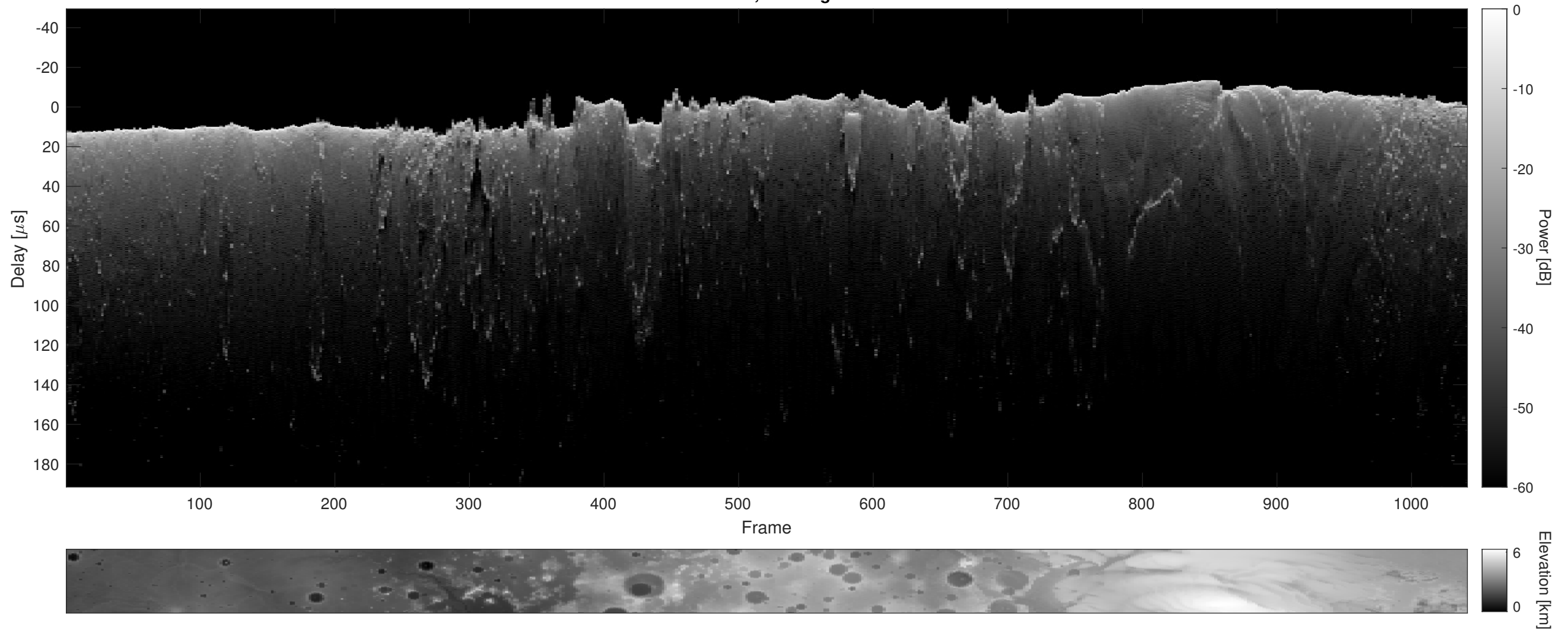
Orbit 6796, Cluttergram
