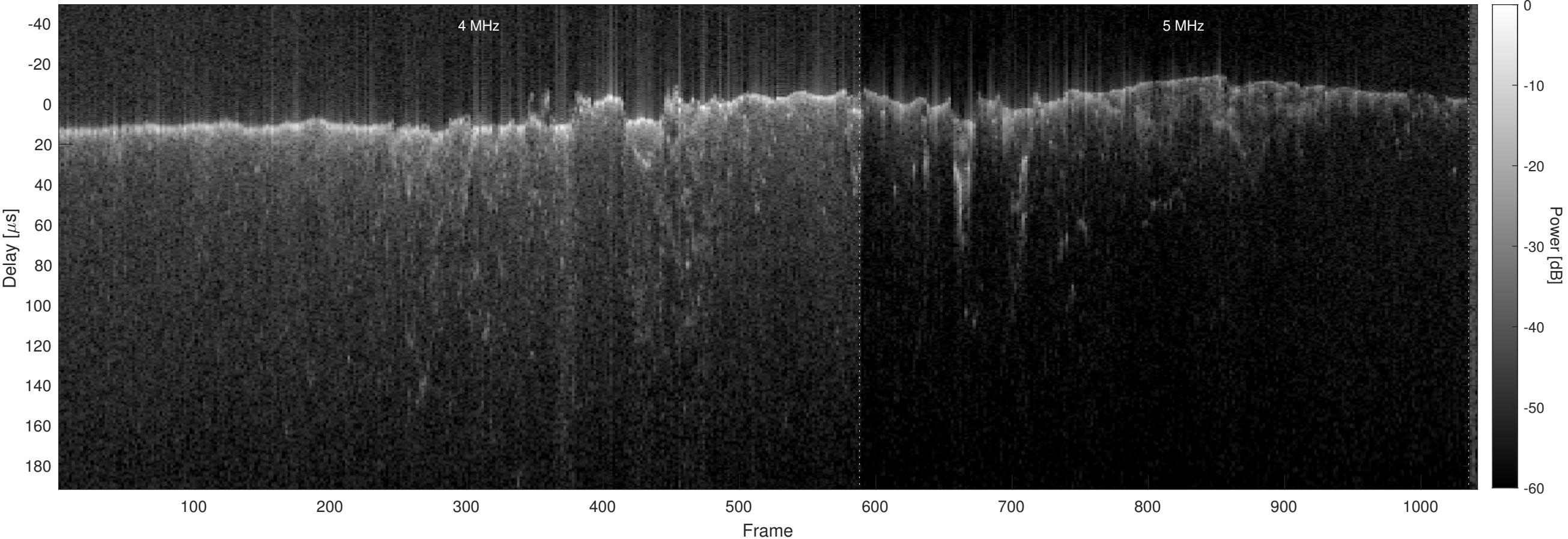
Orbit 6796, Optimized, No Window, Channel 2
