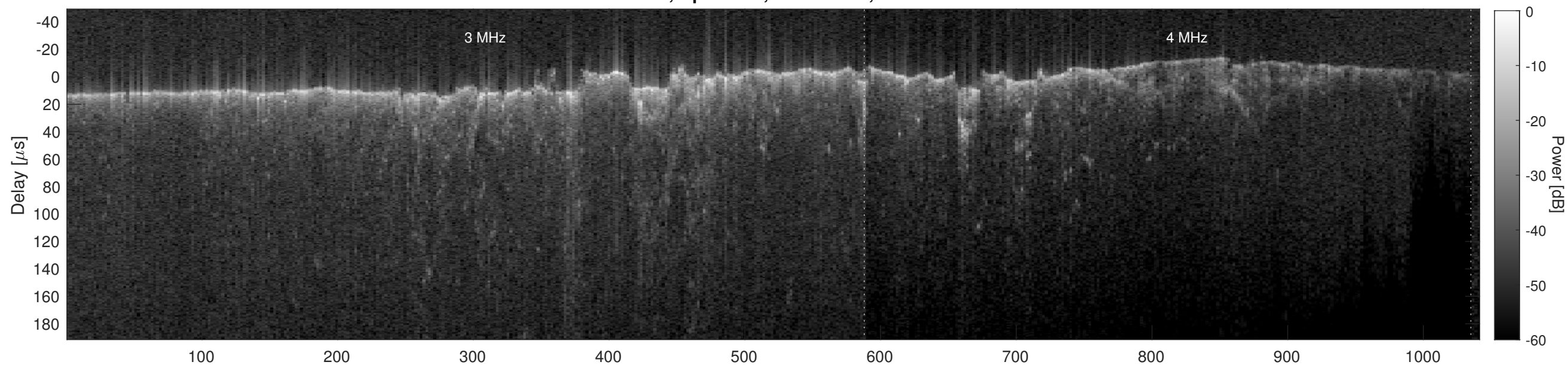
Orbit 6796, Cluttergram
