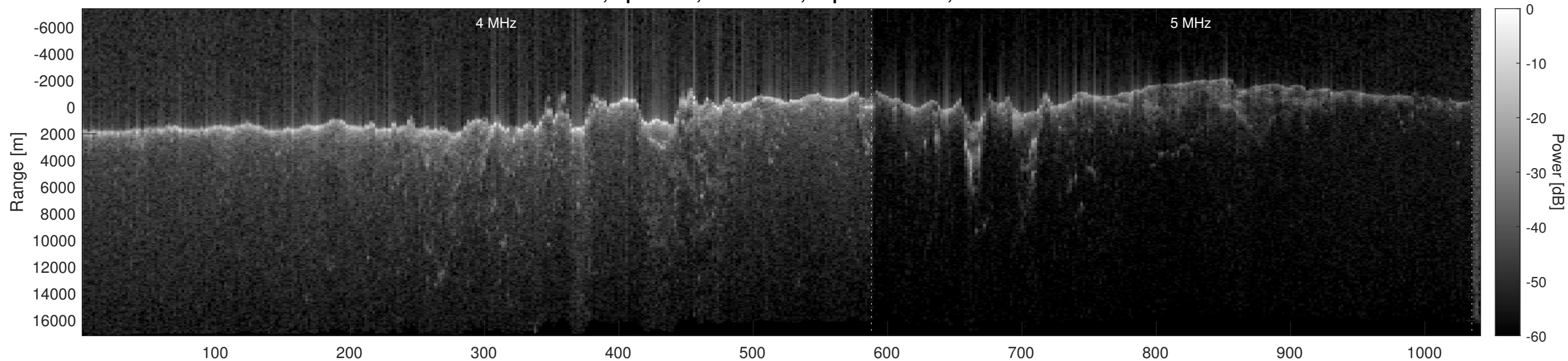
Orbit 6796, Optimized, No Window, Depth-Corrected, Channel 2
