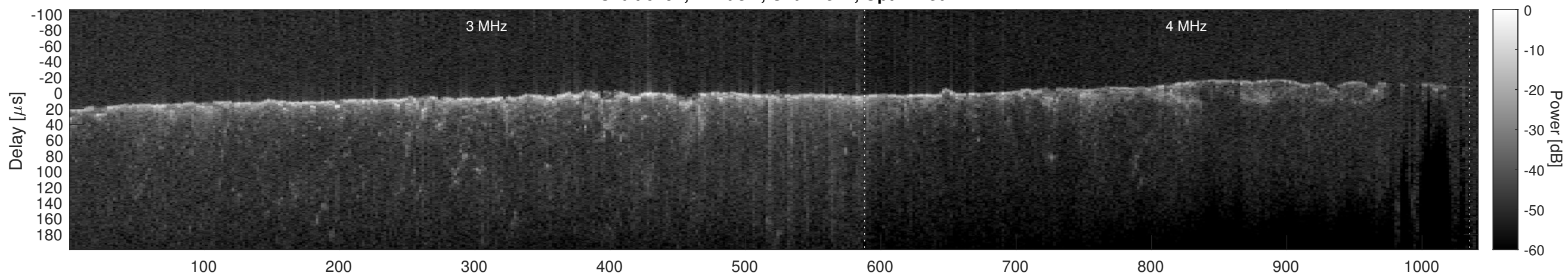
Orbit 6797, Cluttergram
