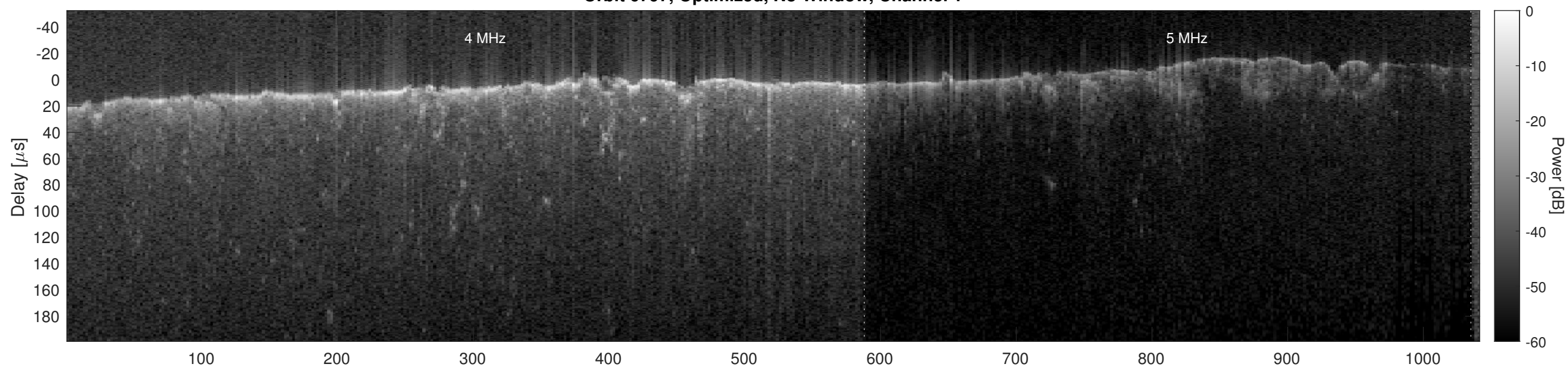
Orbit 6797, Optimized, No Window, Channel 2
