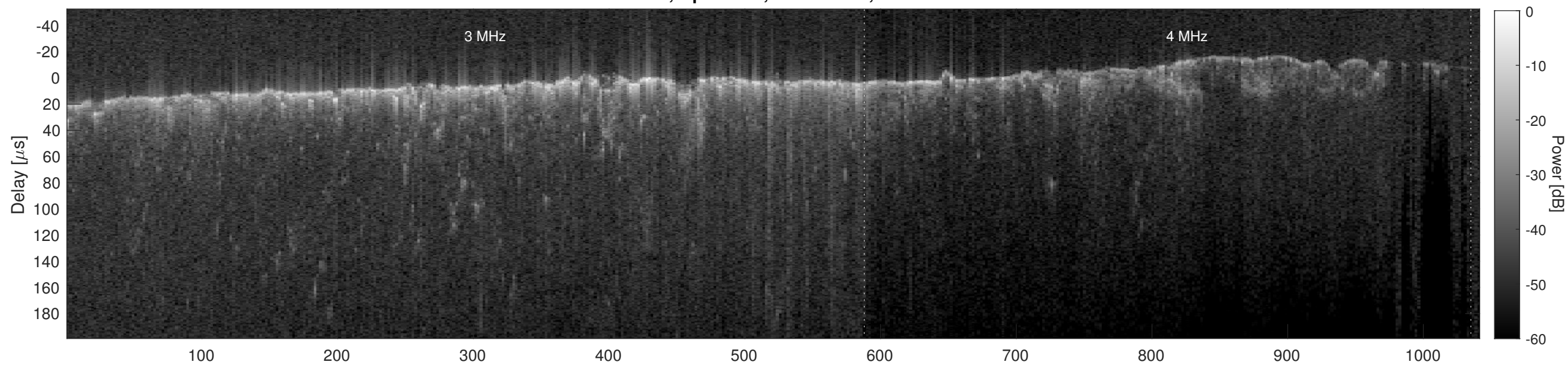
Orbit 6797, Cluttergram
