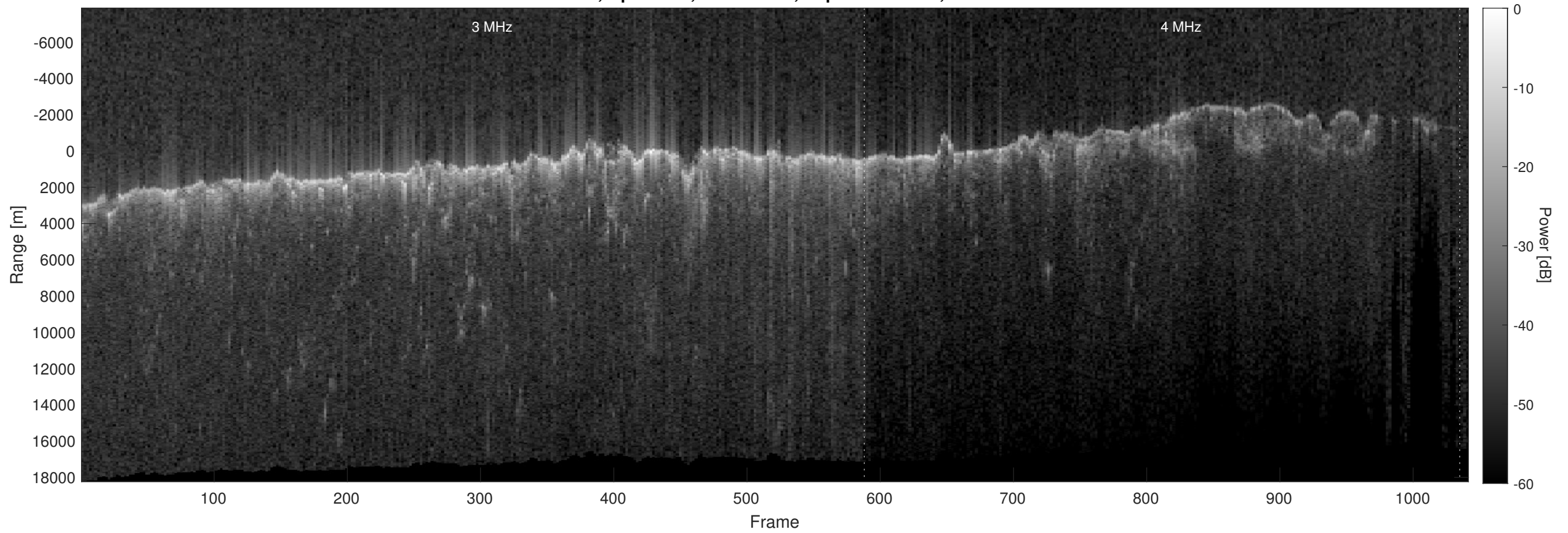
Orbit 6797, Optimized, No Window, Depth-Corrected, Channel 2
