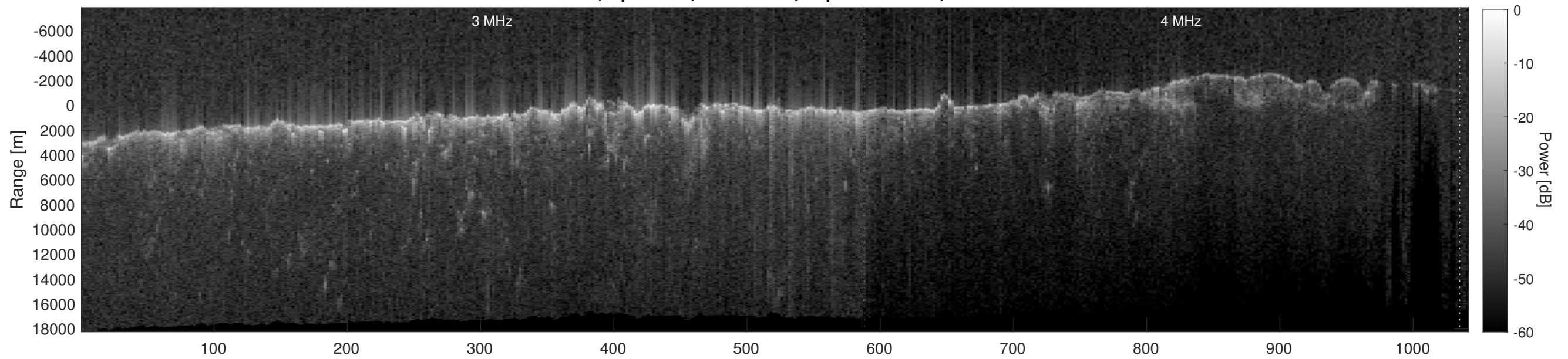
Orbit 6797, Depth-Corrected Cluttergram
