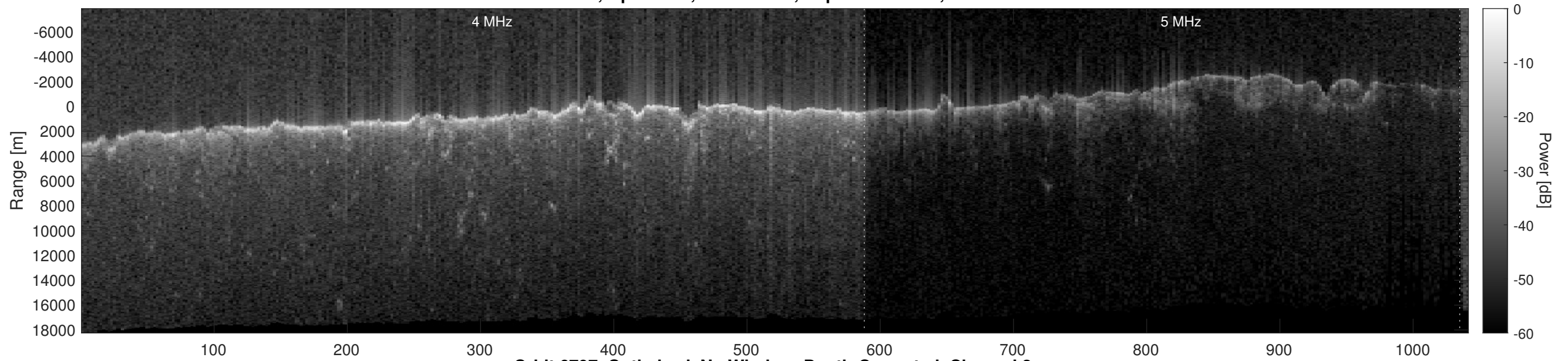
Orbit 6797, Optimized, No Window, Depth-Corrected, Channel 2
