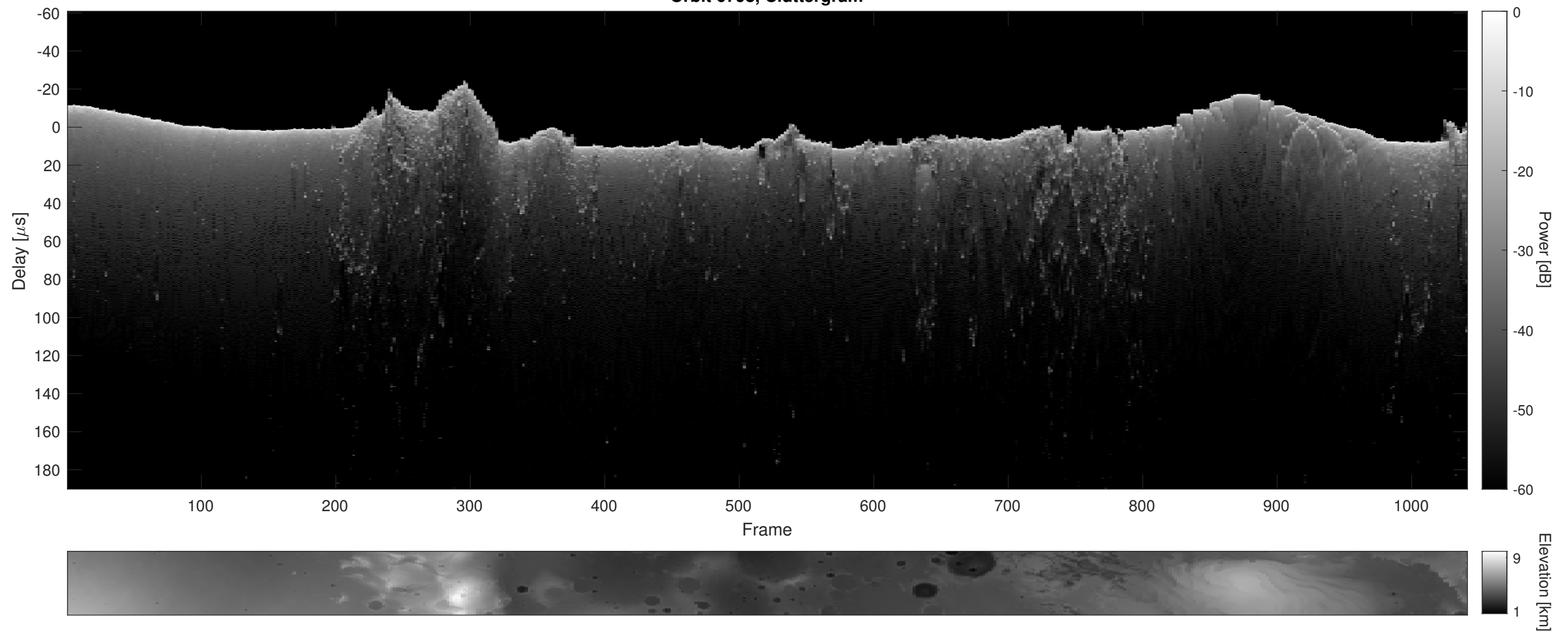
Orbit 6798, Cluttergram
