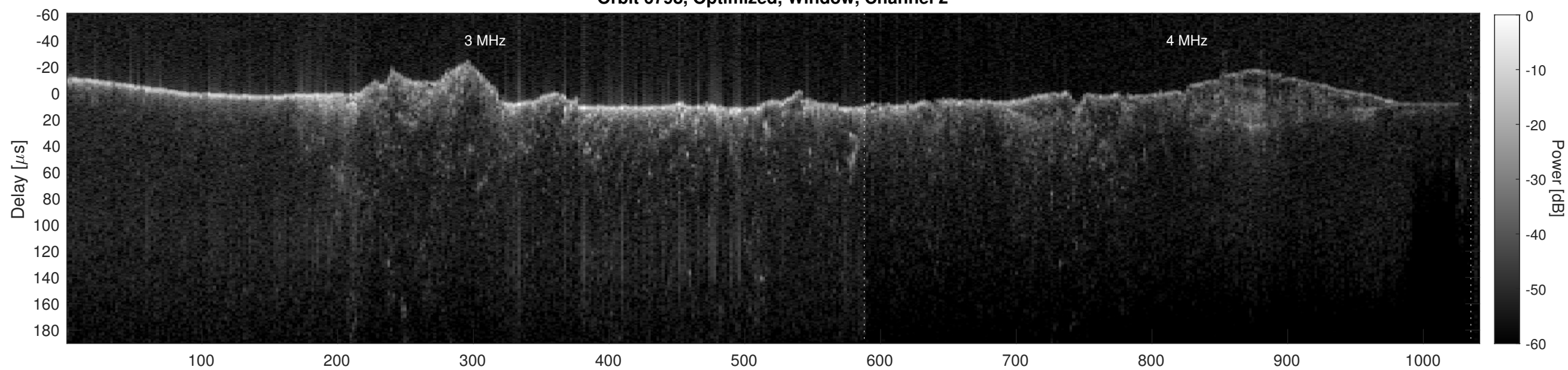
Orbit 6798, Cluttergram
