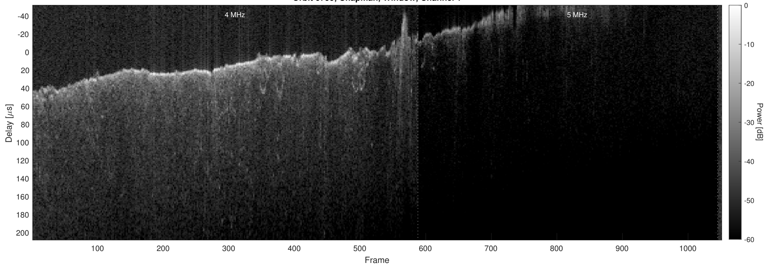
Orbit 6799, Chapman, Window, Channel 2
