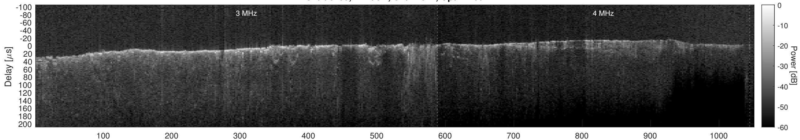
Orbit 6799, Cluttergram
