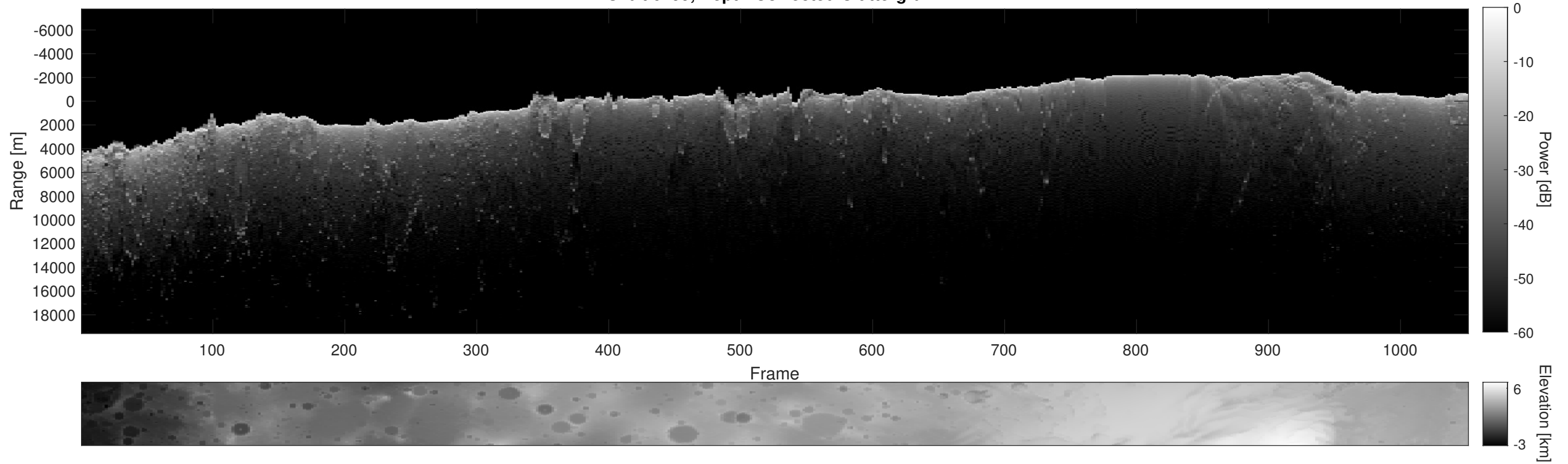
Orbit 6799, Depth-Corrected Cluttergram
