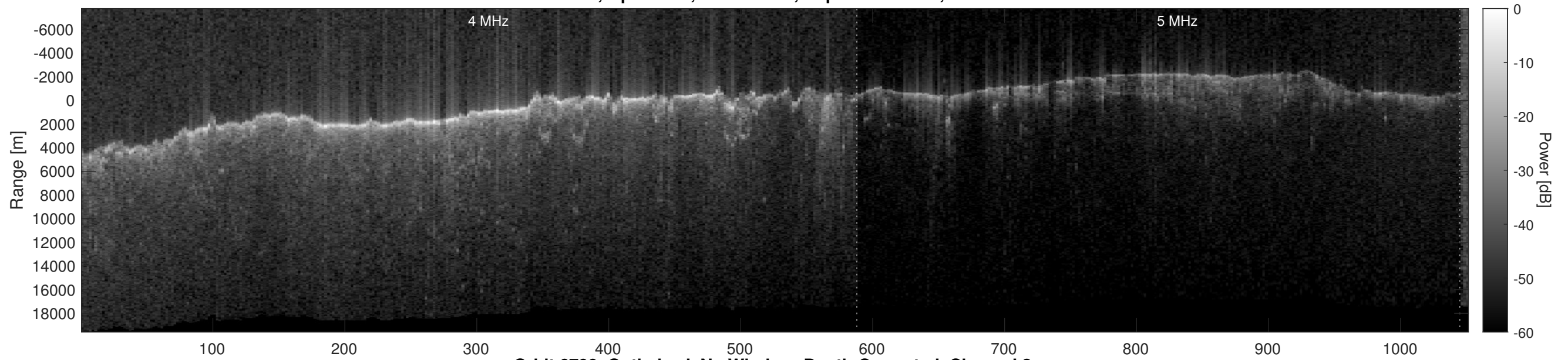
Orbit 6799, Optimized, No Window, Depth-Corrected, Channel 2
