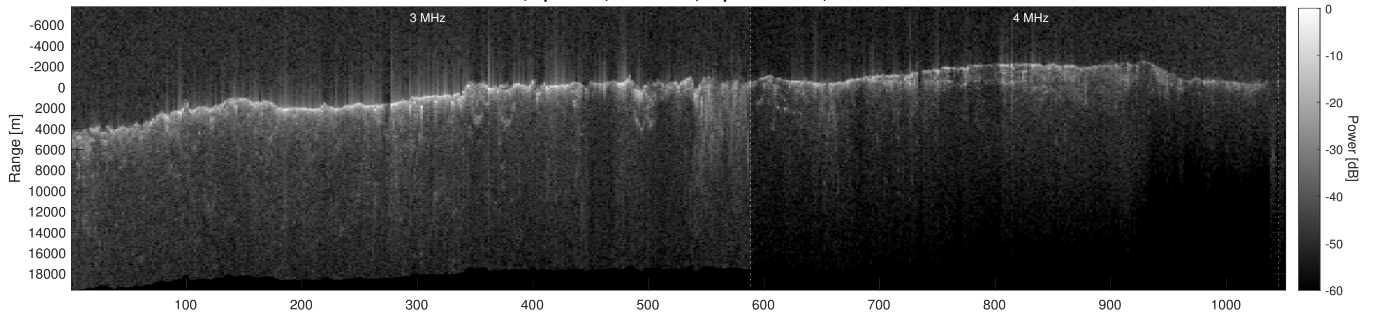
Orbit 6799, Depth-Corrected Cluttergram
