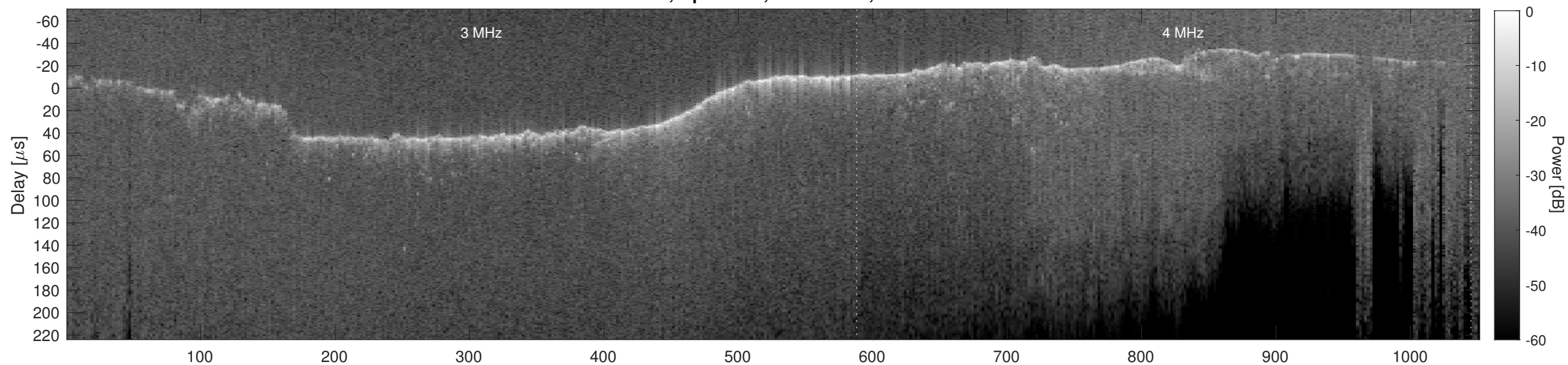
Orbit 6800, Cluttergram
