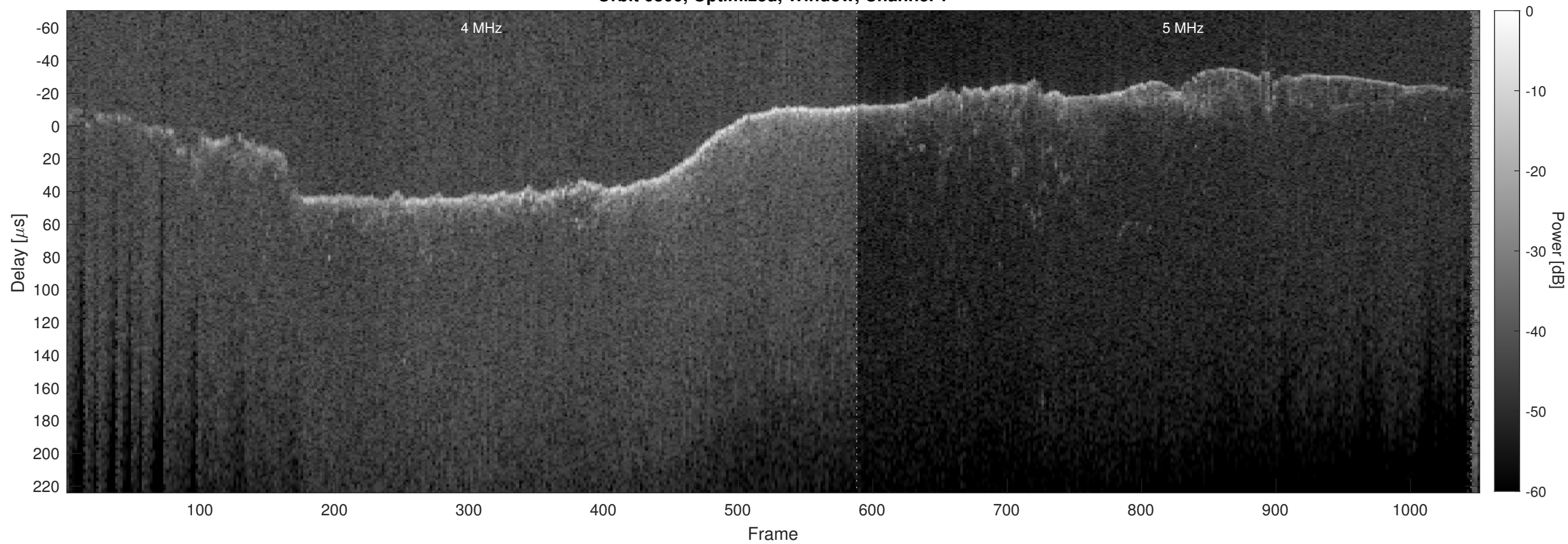
Orbit 6800, Optimized, Window, Channel 2
