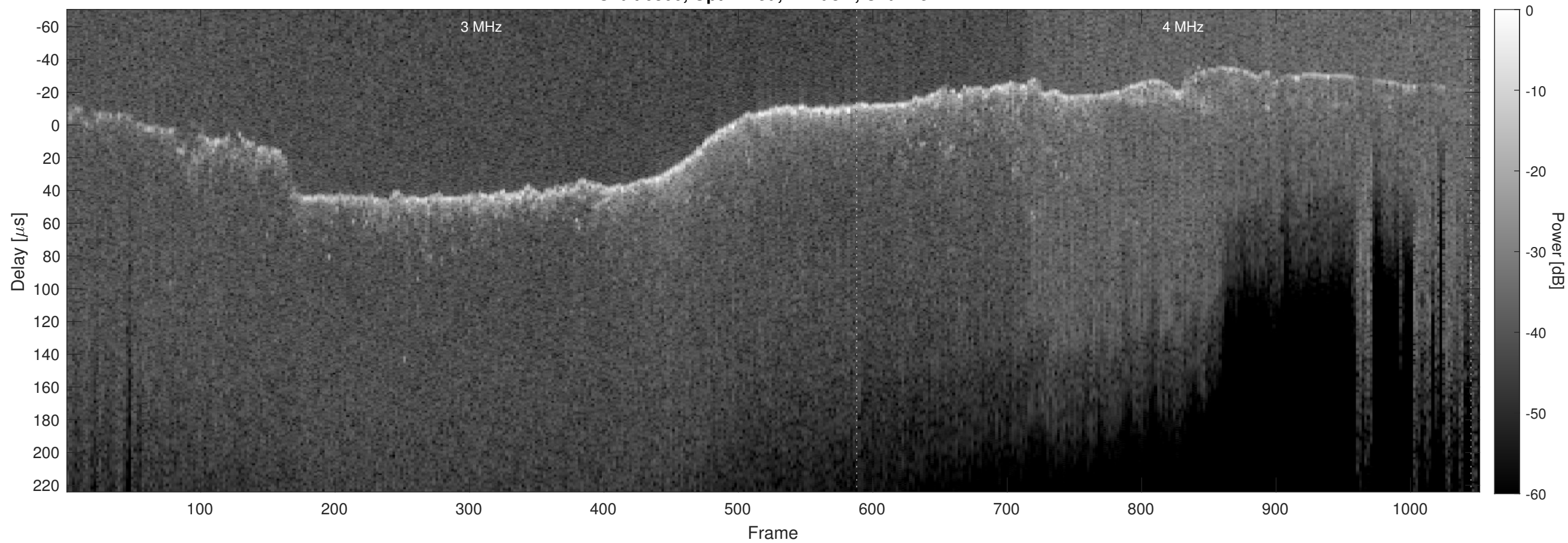
Orbit 6800, Optimized, Window, Channel 2
