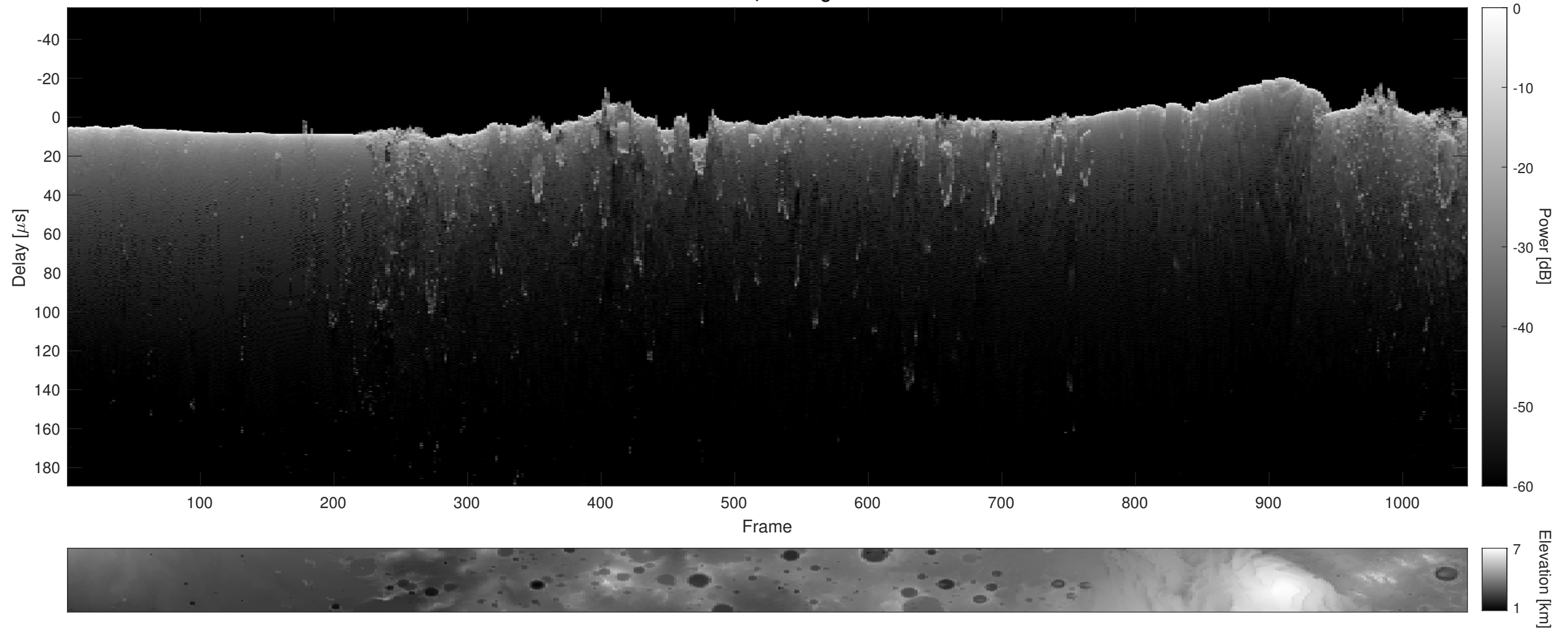
Orbit 6802, Cluttergram
