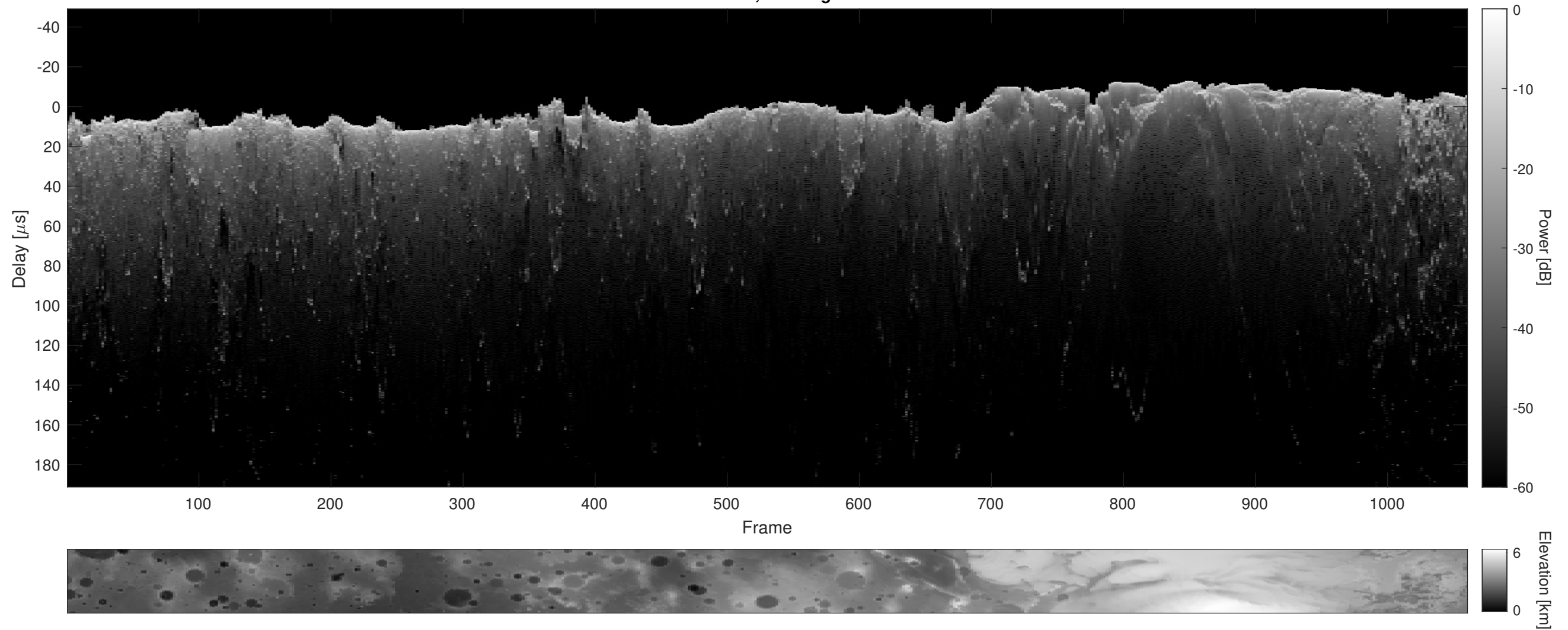
Orbit 6803, Cluttergram
