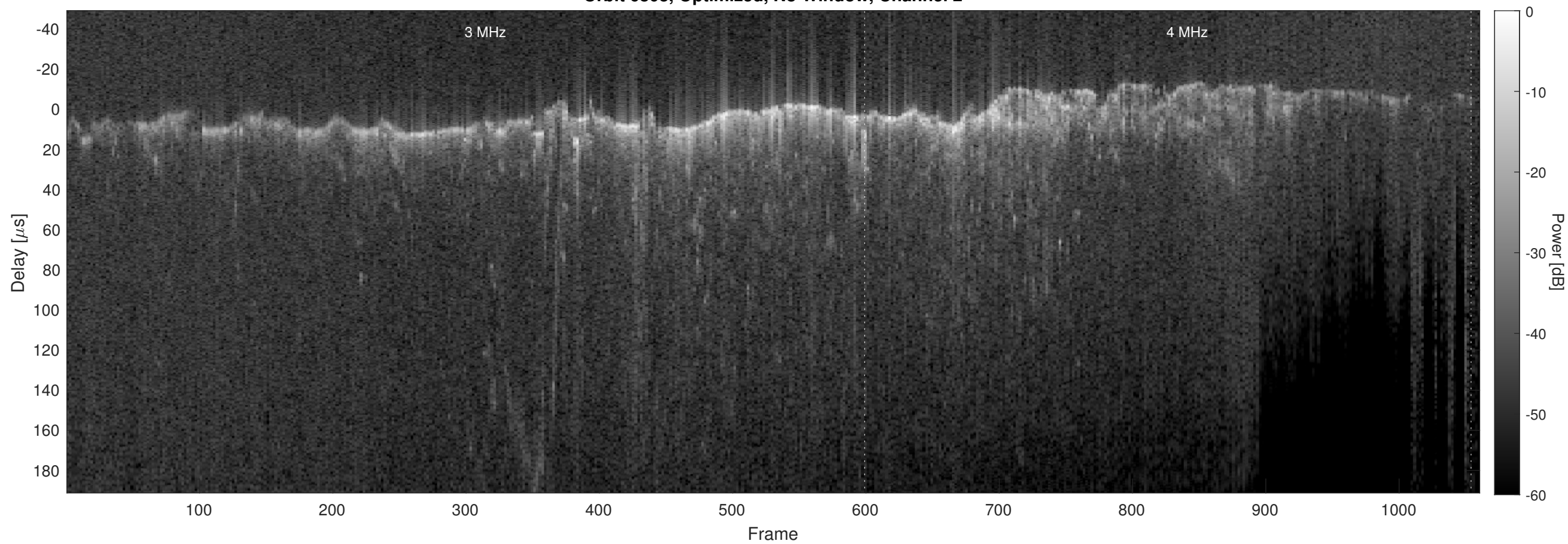
Orbit 6803, Optimized, No Window, Channel 2
