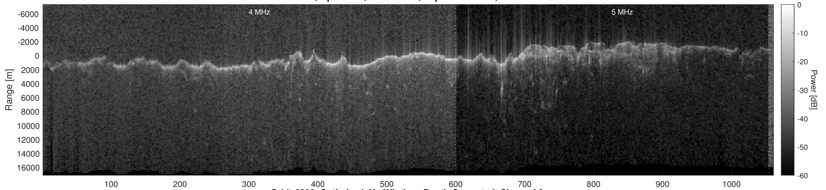
Orbit 6803, Optimized, No Window, Depth-Corrected, Channel 2
