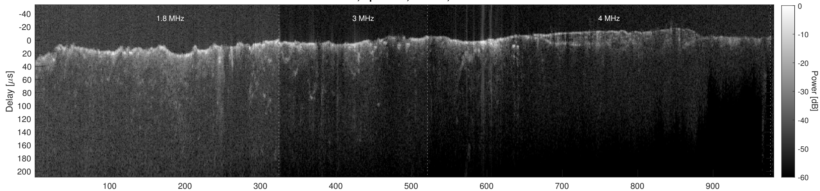
Orbit 6806, Cluttergram
