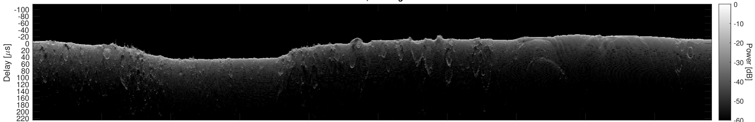
Orbit 6807, Cluttergram
