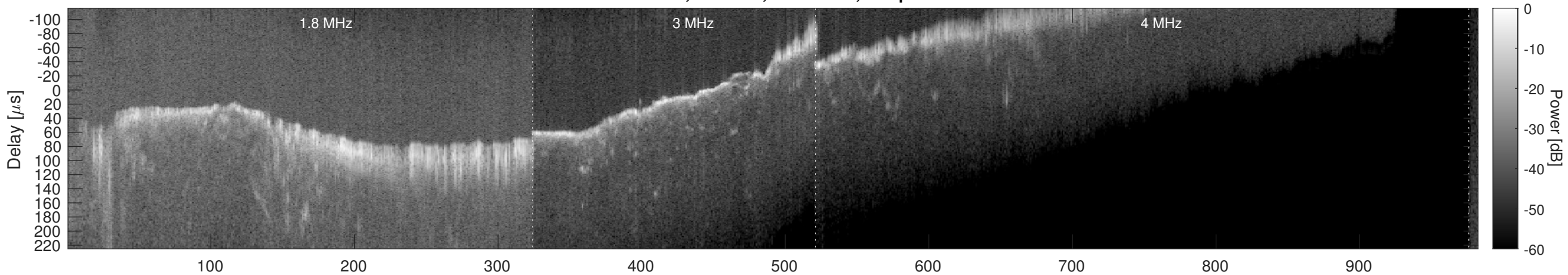
Orbit 6807, Window, Channel 2, Optimized
