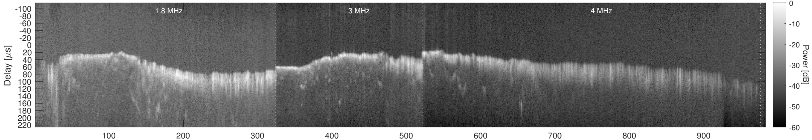
Orbit 6807, Window, Channel 2, Chapman
