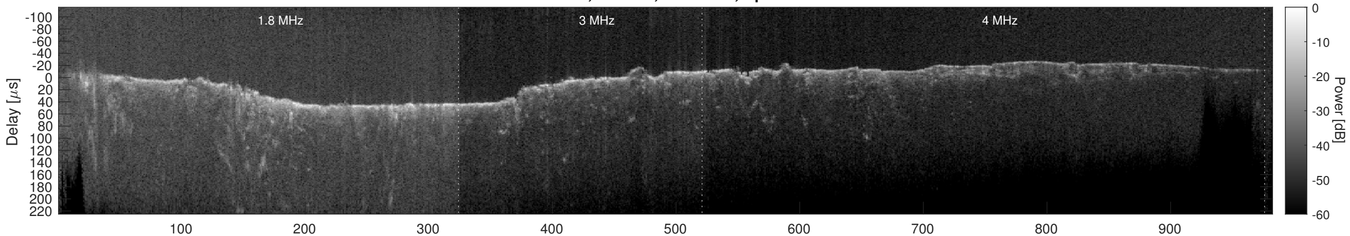
Orbit 6807, Cluttergram
