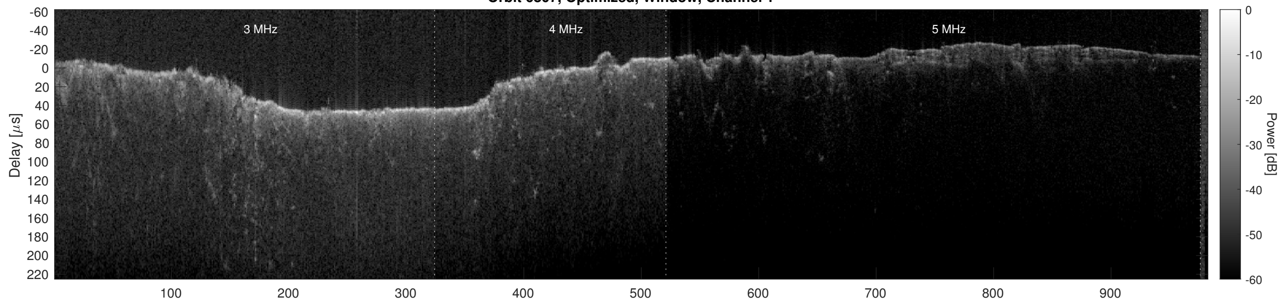
Orbit 6807, Optimized, Window, Channel 2
