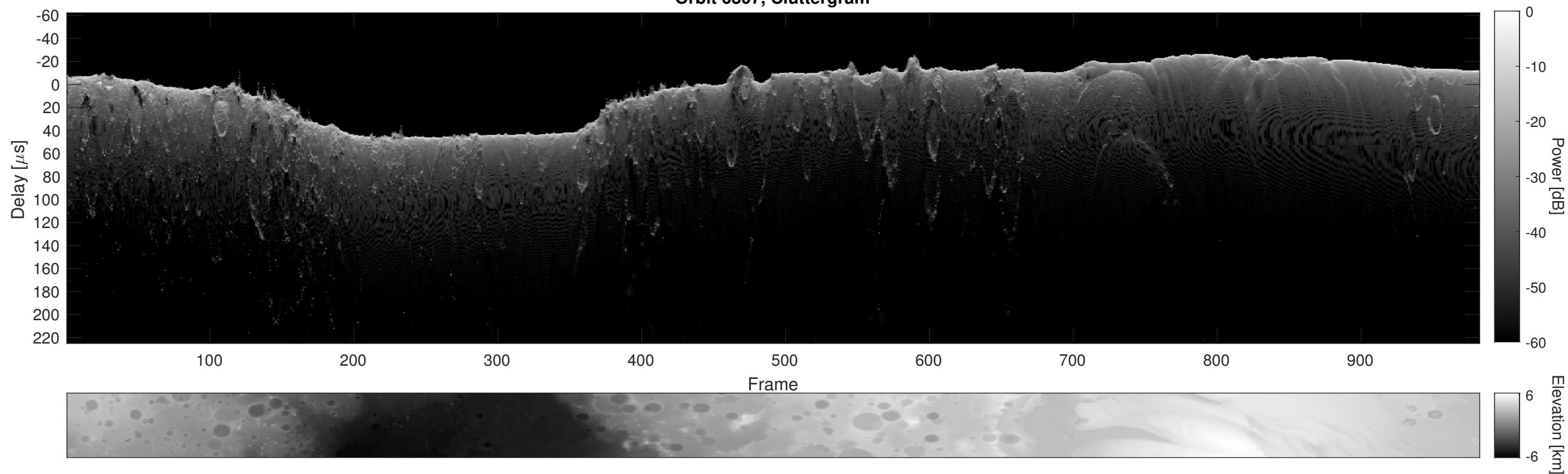
Orbit 6807, Cluttergram
