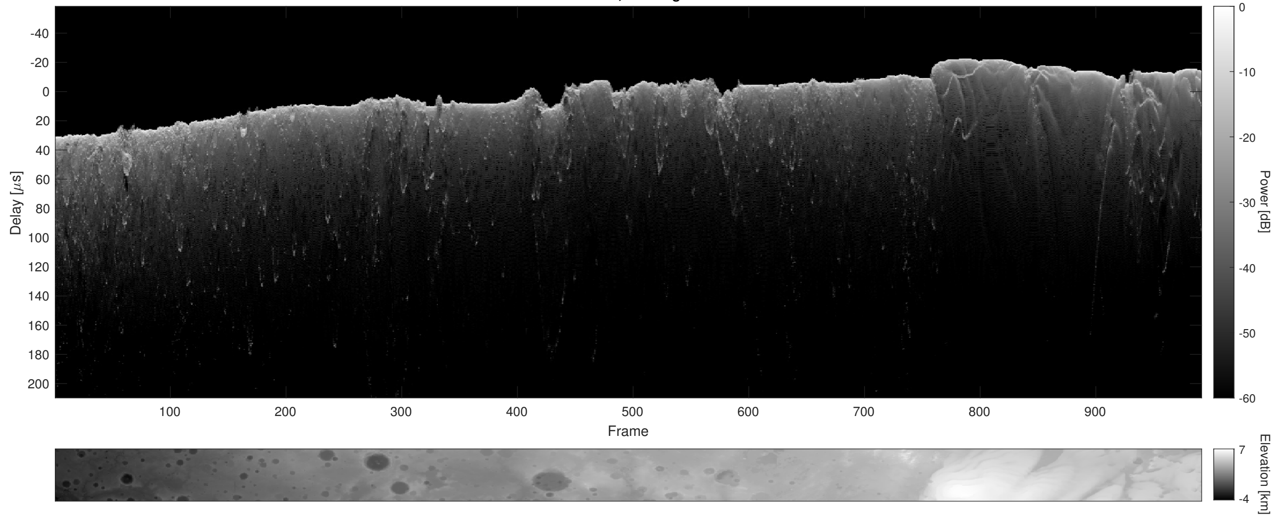
Orbit 6808, Cluttergram
