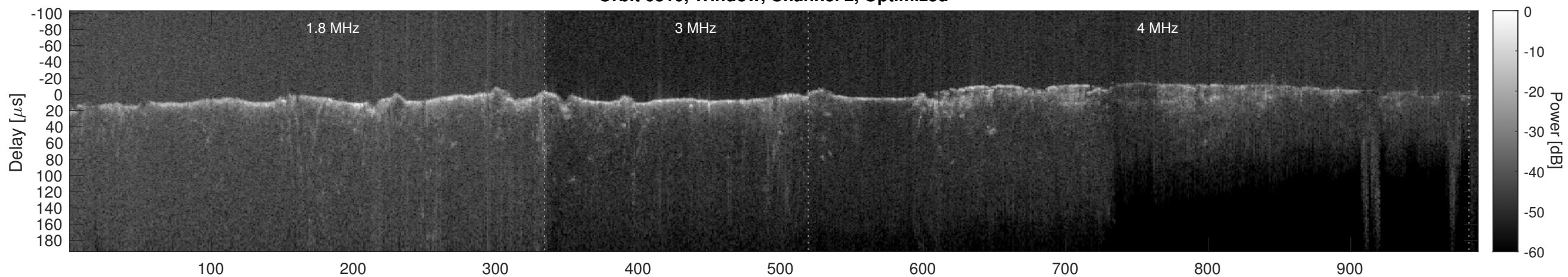
Orbit 6810, Cluttergram
