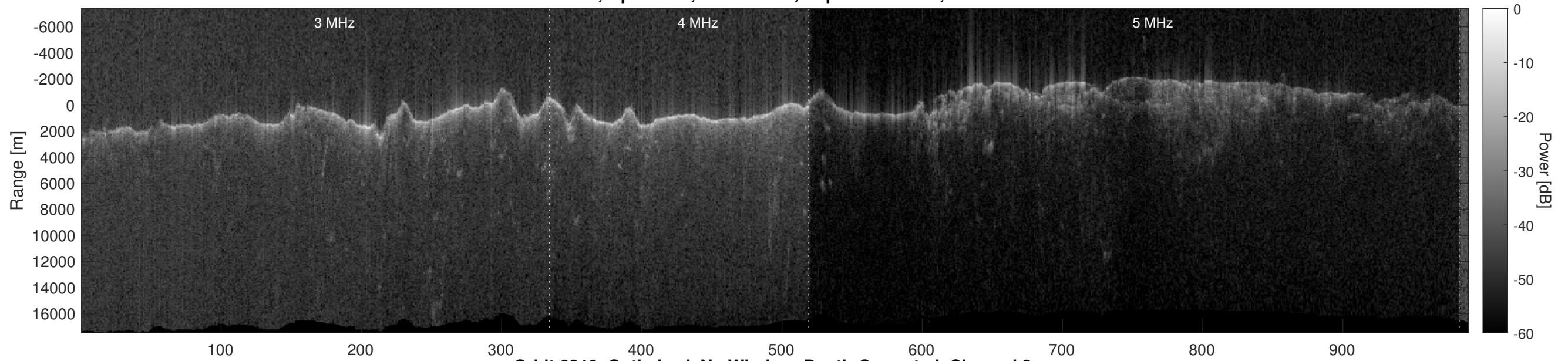
Orbit 6810, Optimized, No Window, Depth-Corrected, Channel 2
