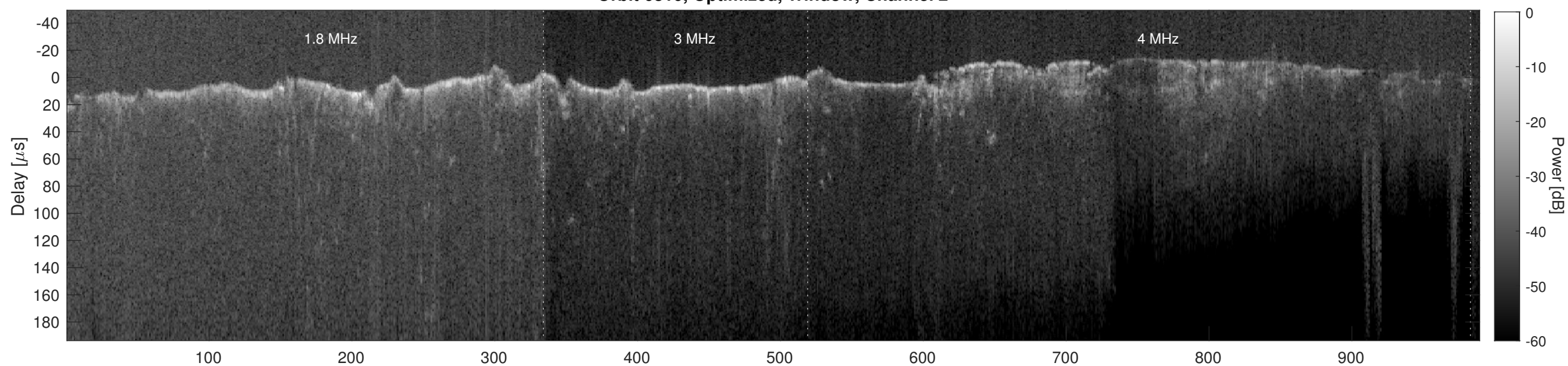
Orbit 6810, Cluttergram
