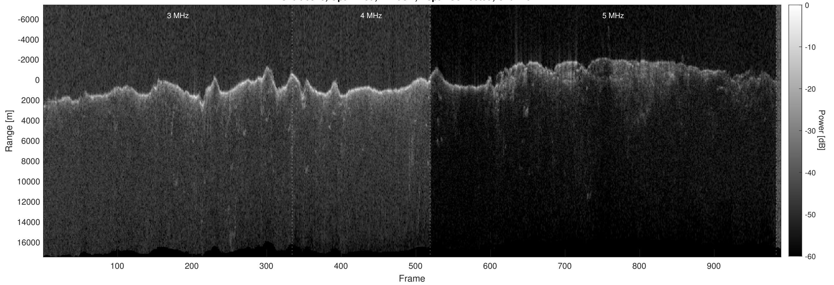
Orbit 6810, Optimized, Window, Depth-Corrected, Channel 2
