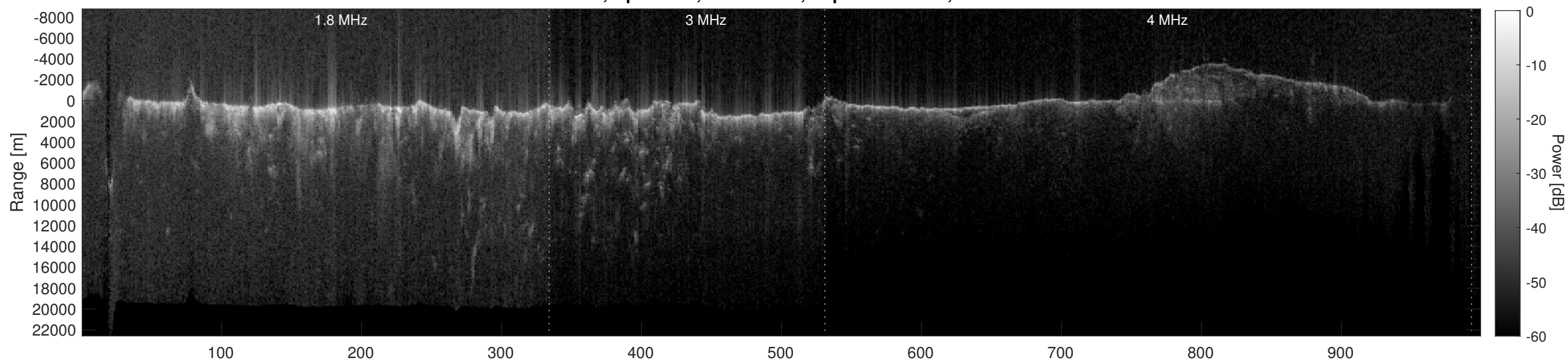
Orbit 6812, Depth-Corrected Cluttergram
