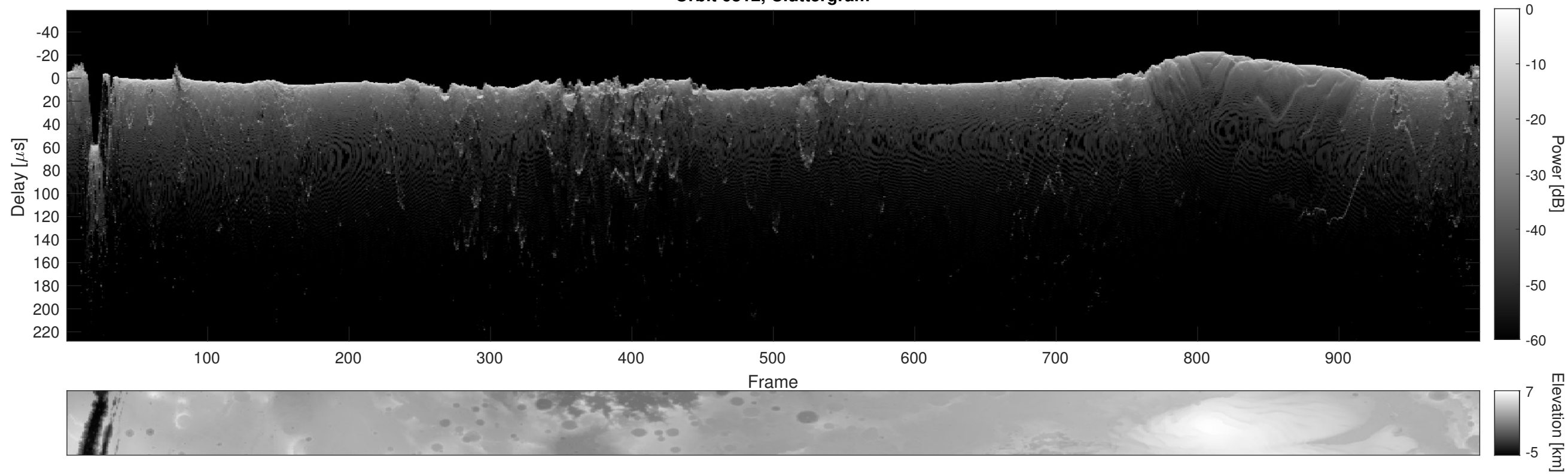
Orbit 6812, Cluttergram
