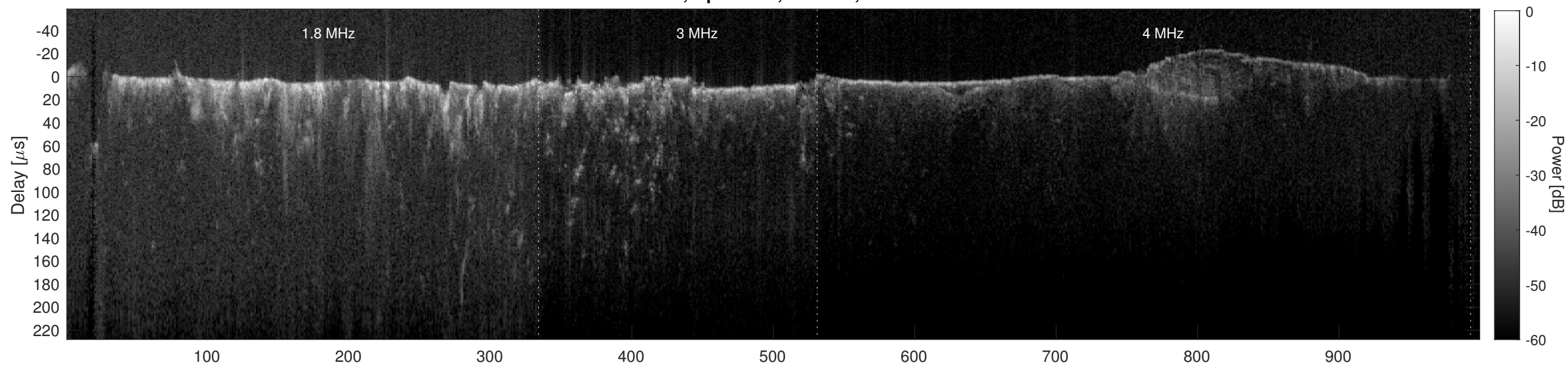
Orbit 6812, Cluttergram
