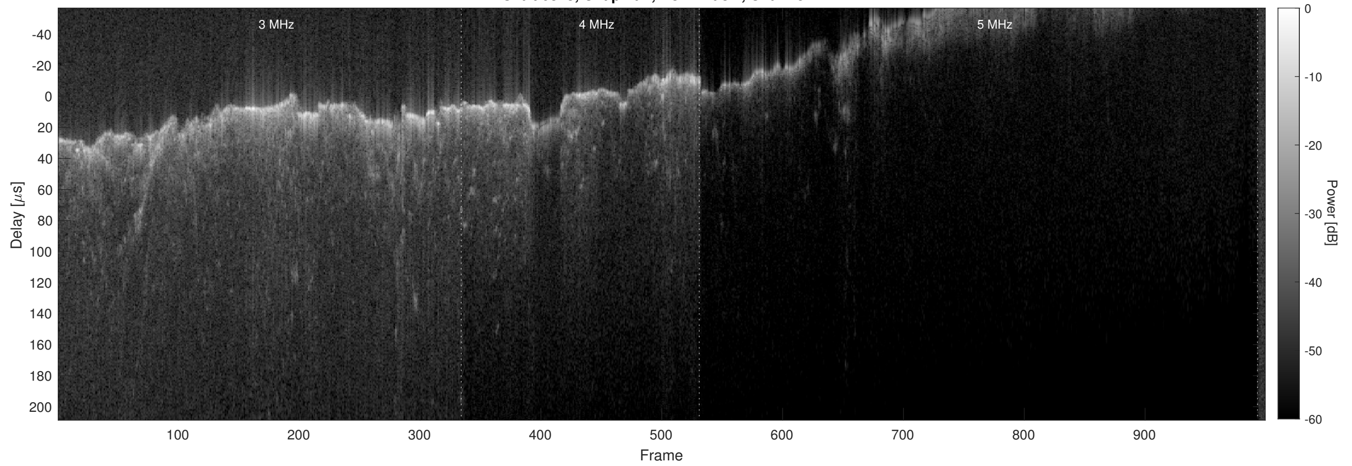
Orbit 6813, Chapman, No Window, Channel 2
