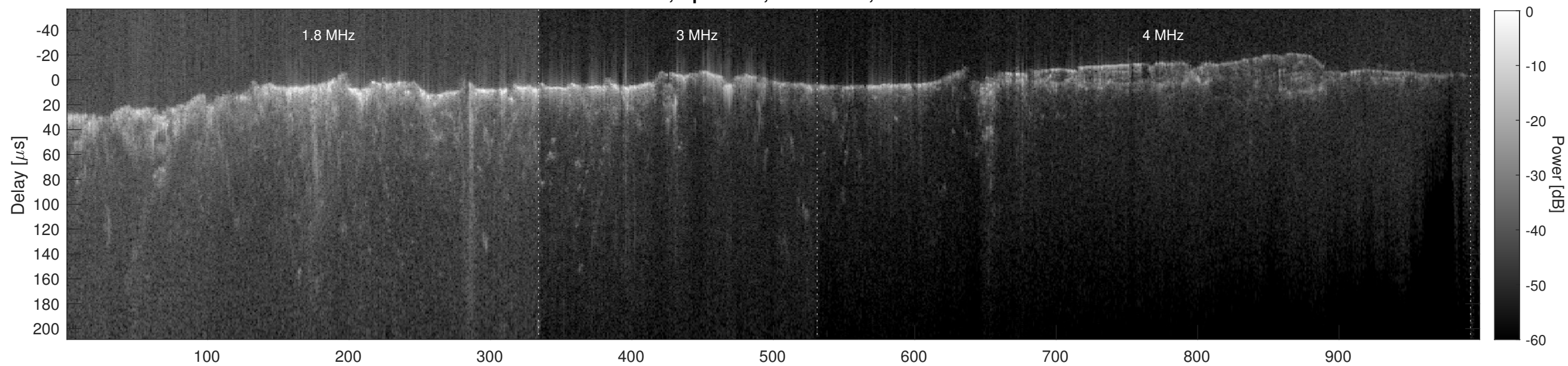
Orbit 6813, Cluttergram
