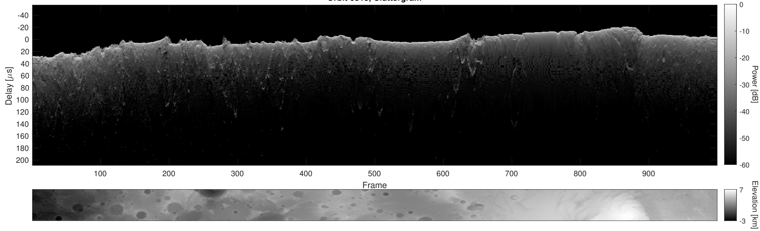
Orbit 6813, Cluttergram
