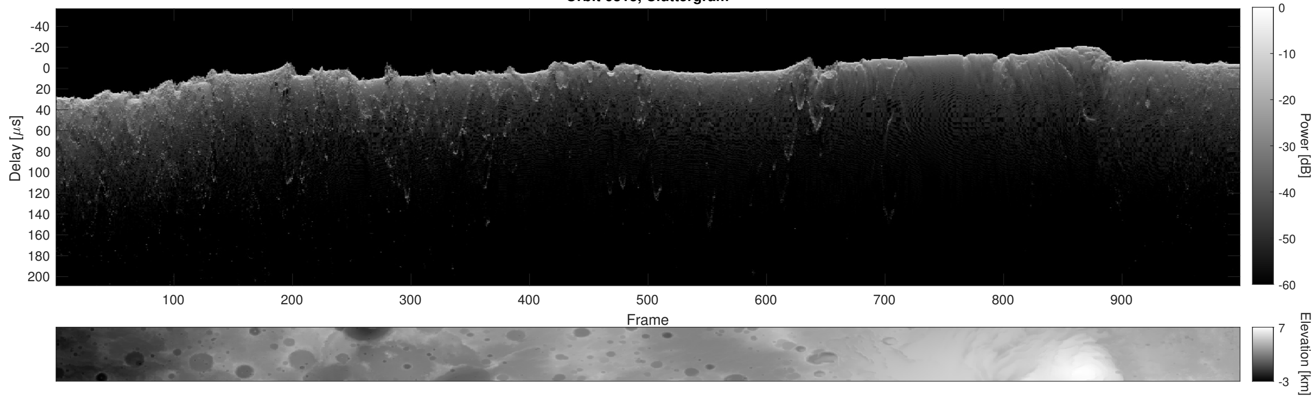
Orbit 6813, Cluttergram
