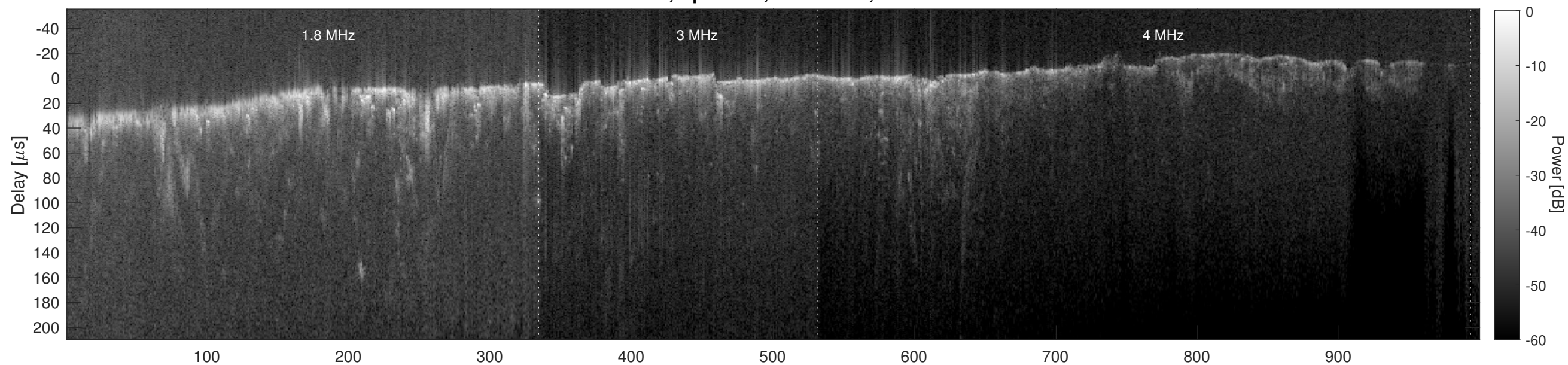
Orbit 6815, Cluttergram
