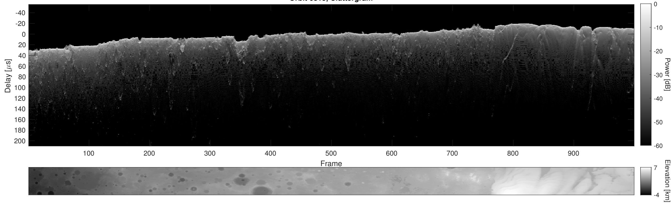
Orbit 6815, Cluttergram
