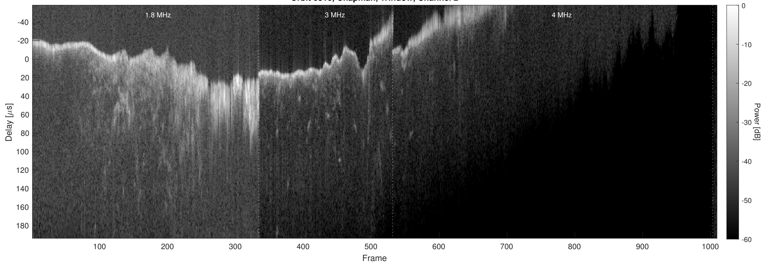
Orbit 6816, Chapman, Window, Channel 2
