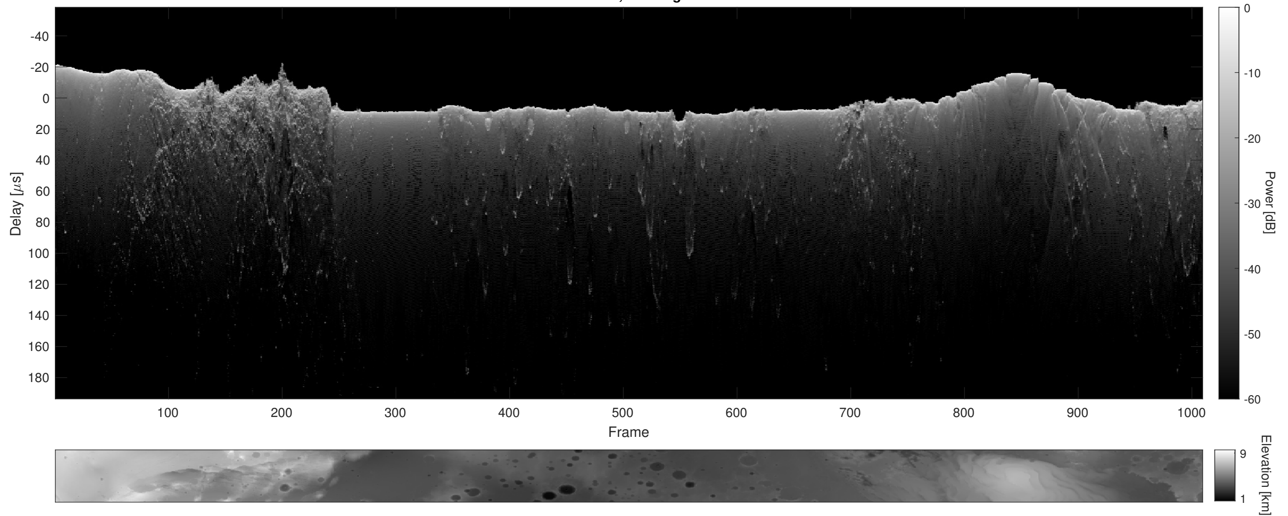
Orbit 6816, Cluttergram
