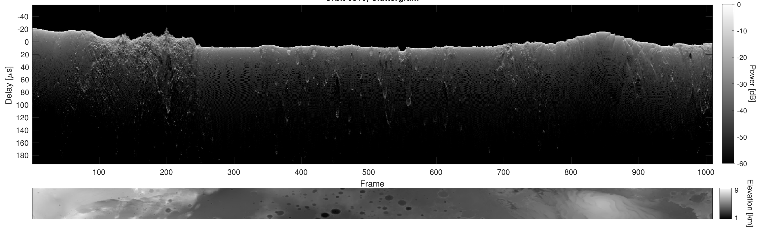
Orbit 6816, Cluttergram
