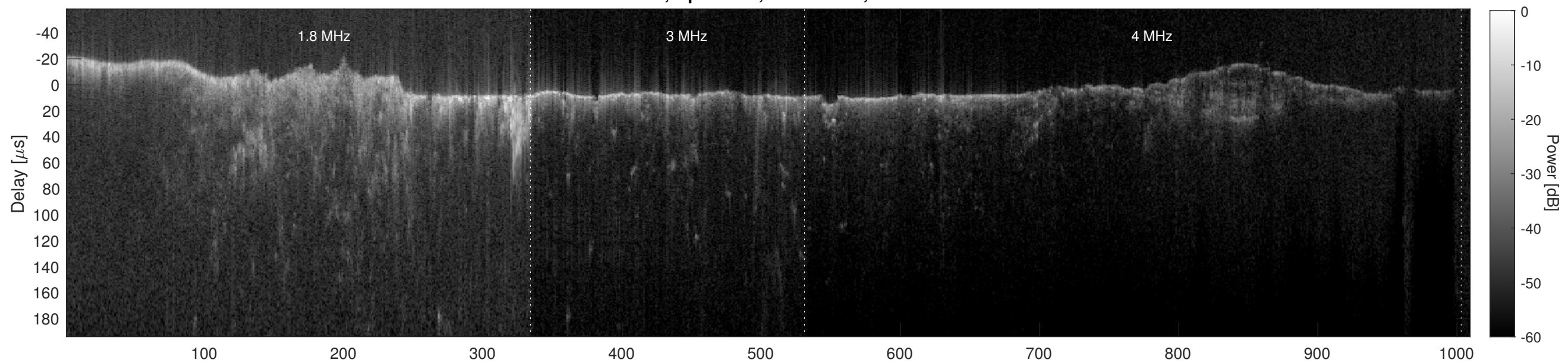
Orbit 6816, Cluttergram
