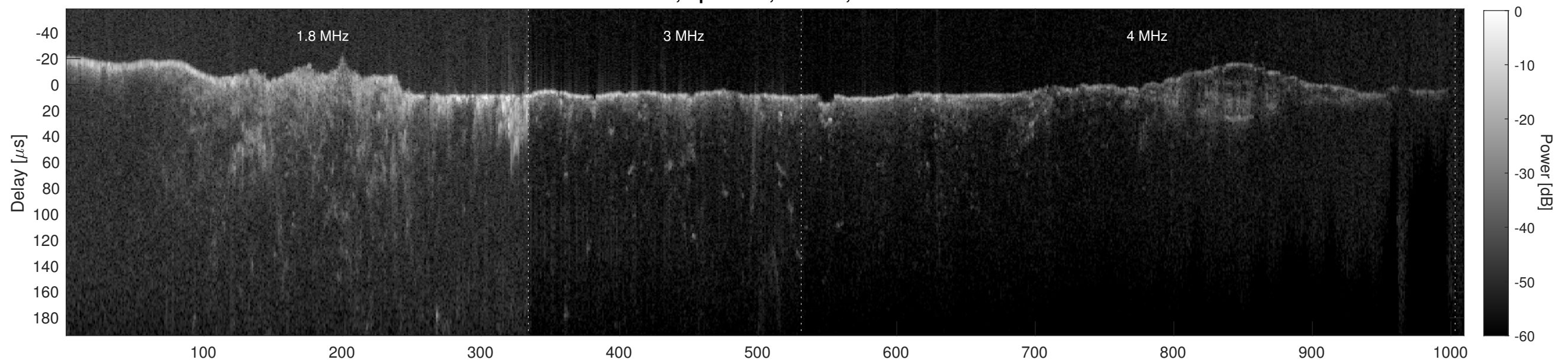
Orbit 6816, Cluttergram
