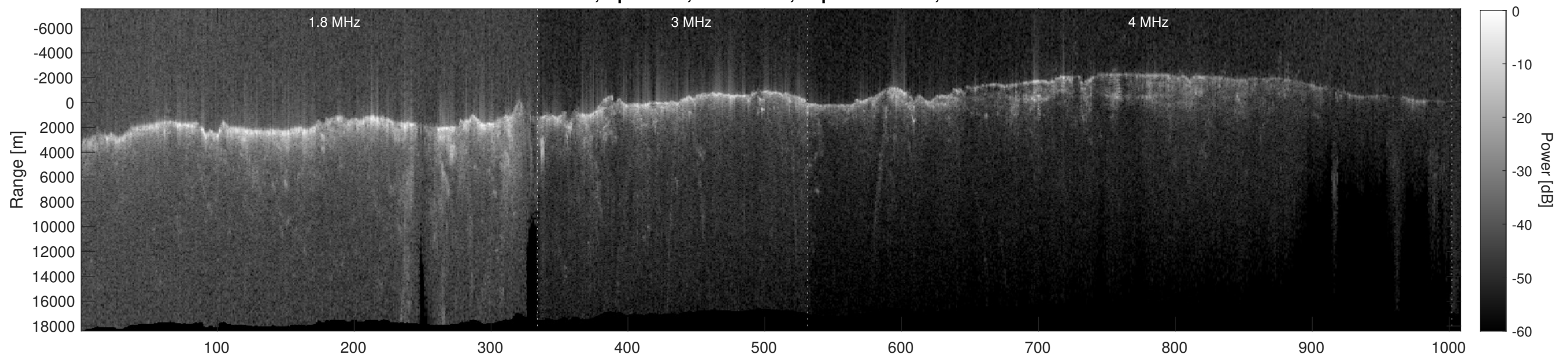
Orbit 6817, Depth-Corrected Cluttergram
