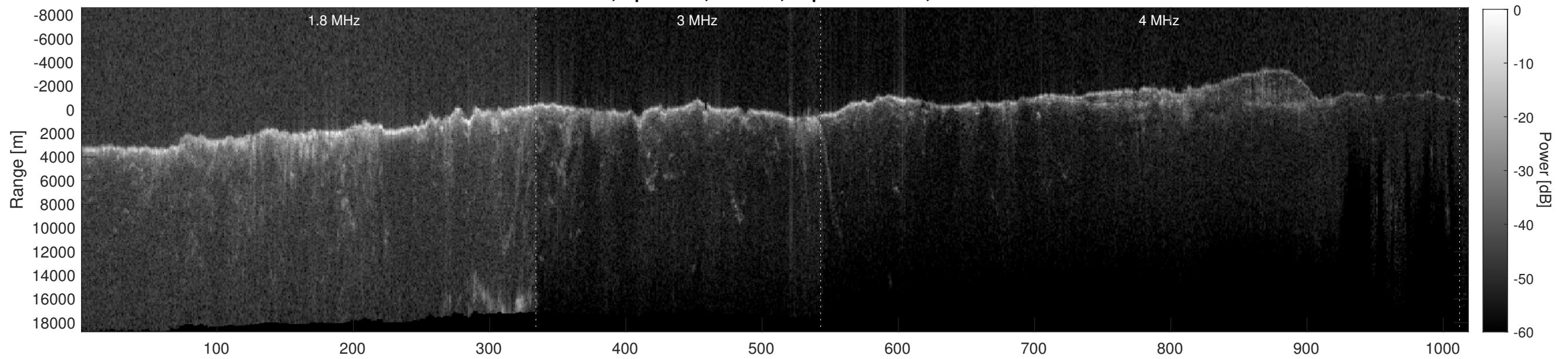
Orbit 6820, Depth-Corrected Cluttergram
