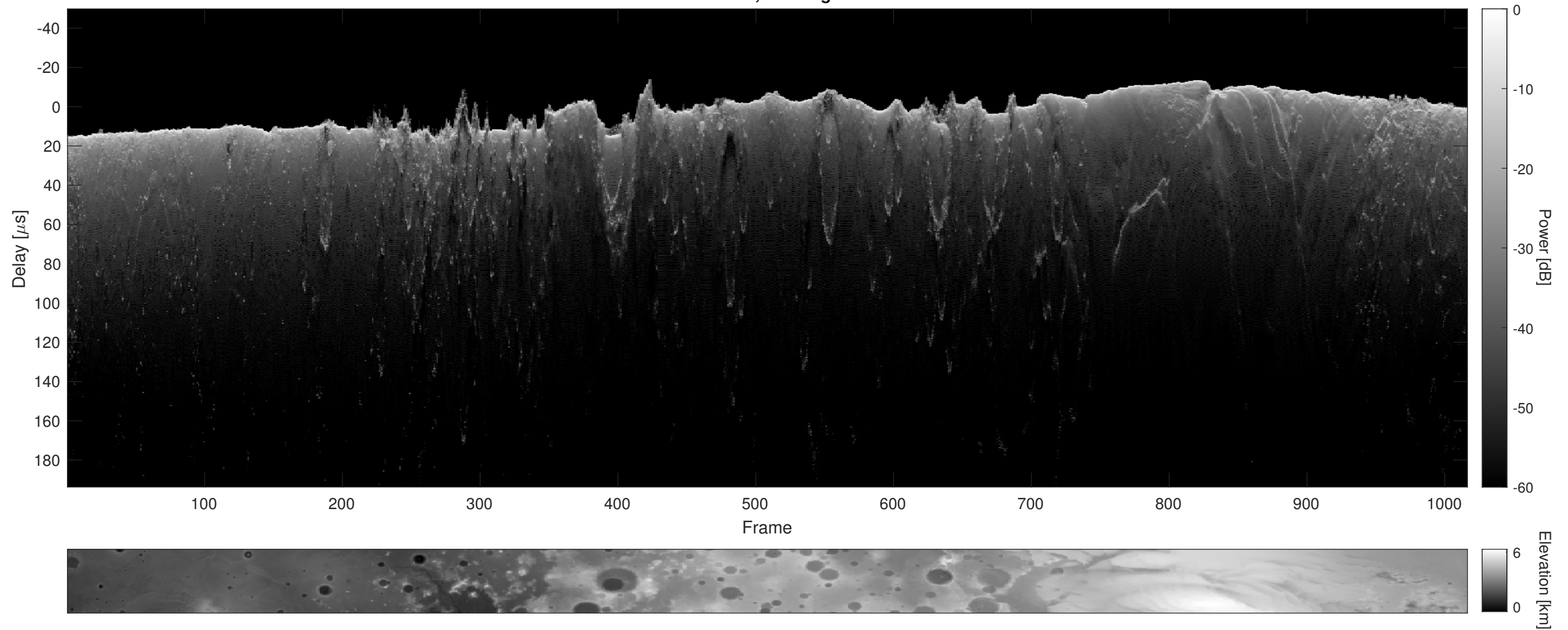
Orbit 6821, Cluttergram
