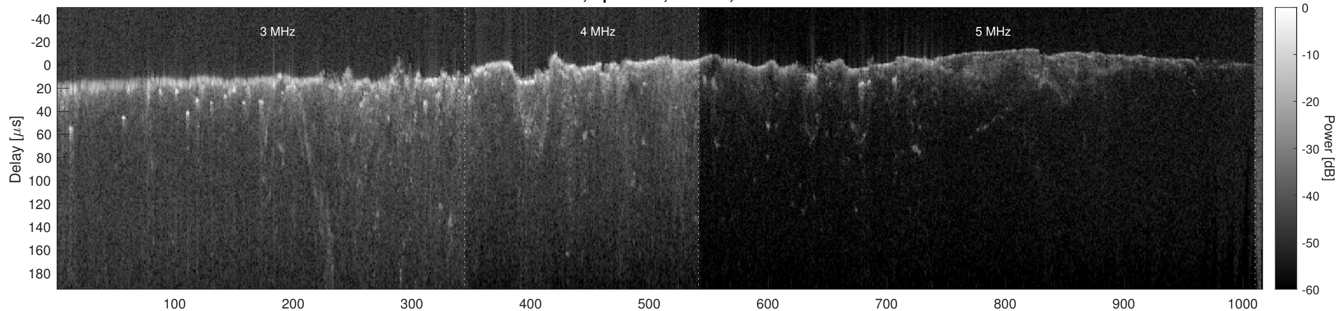
Orbit 6821, Optimized, Window, Channel 2
